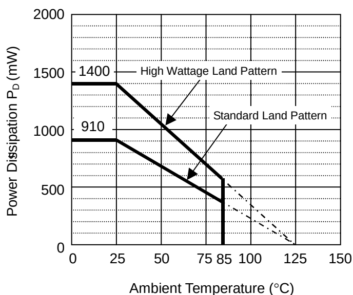
Power Dissipation
