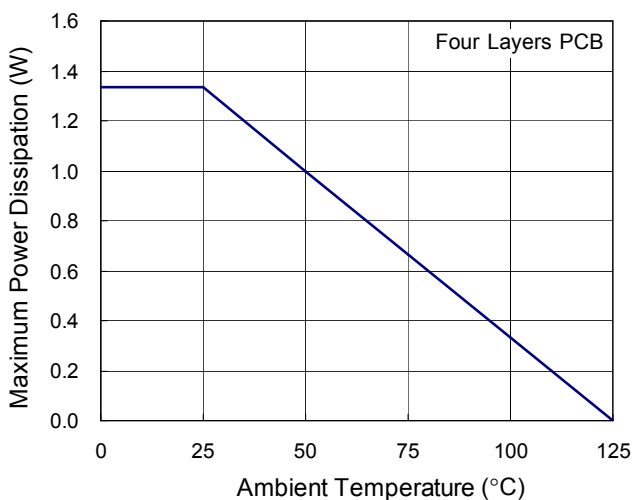
Figure 3. Derating Curve for RP6002 Package
