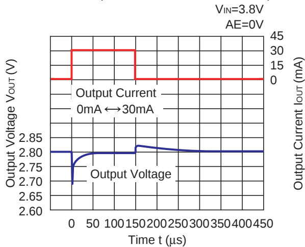
RP201x28xx Auto ECO (Low Power Mode \leftrightarrow Fast Mode)
