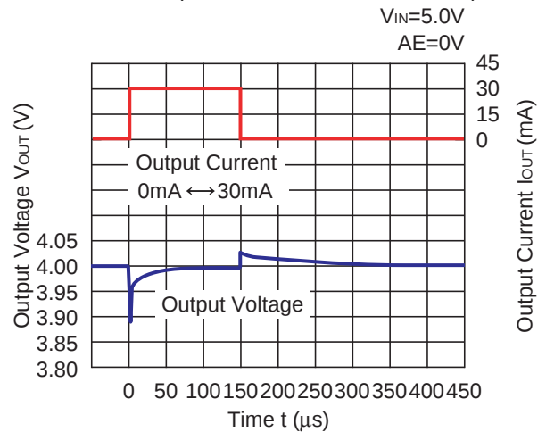
RP201x40xx Auto ECO (Low Power Mode \leftrightarrow Fast Mode)
