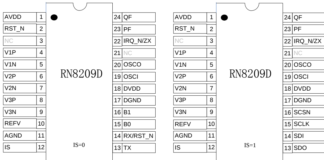
Figure 1-2 RN8209D-SSOP24 Pin Assignment
