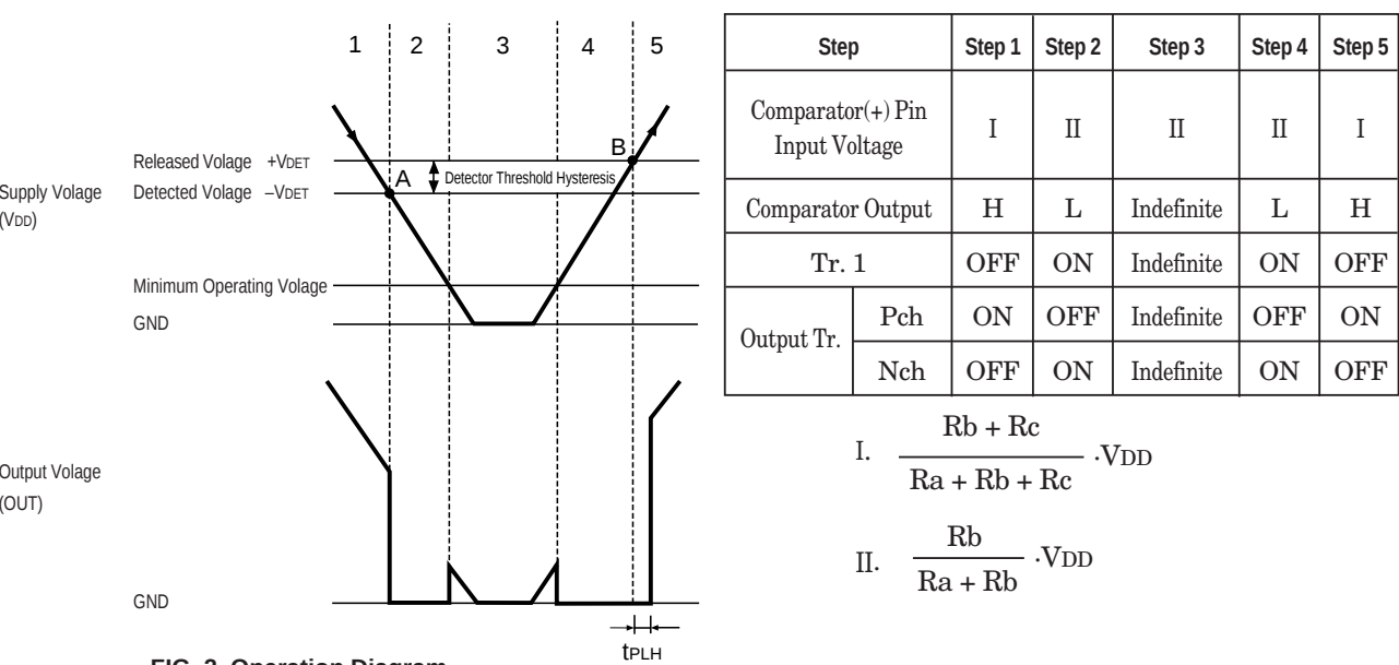
FIG. 2 Operation Diagram
