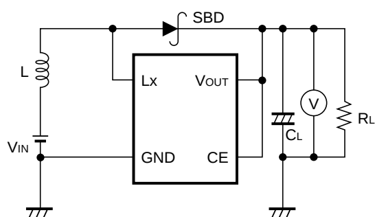
Test Circuit 1
