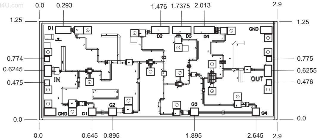
Figure 2. Chip Layout and Bond Pad Locations (Chip Size is 2.9mm x 1.25mm x 100µm. Back of chip is RF and DC Ground)
