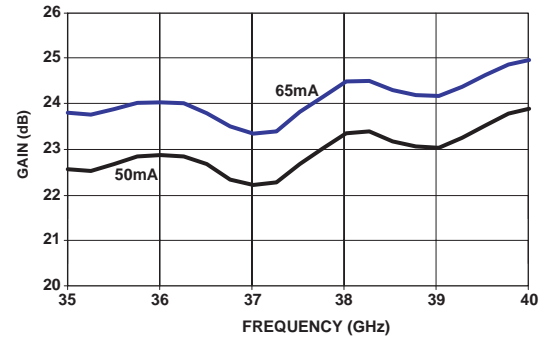
RMWL38001, 37–40GHz Low-Noise Amplifier, Typical Performance, Vd = 4V, Idq = 50mA and 65mA, Chip Bonded into 50Ω Test Fixture
