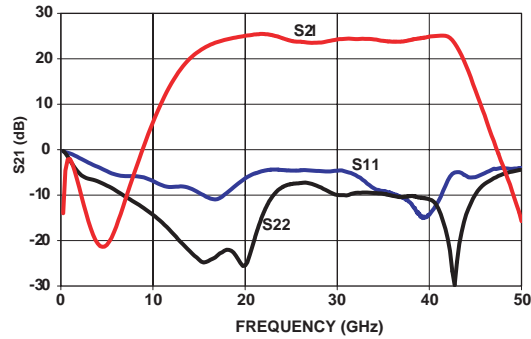
RMWL38001, 37–40GHz Low-Noise Amplifier, Typical Performance, Vd = 4V, Idq = 50mA, Chip Bonded into 50Ω Test Fixture
