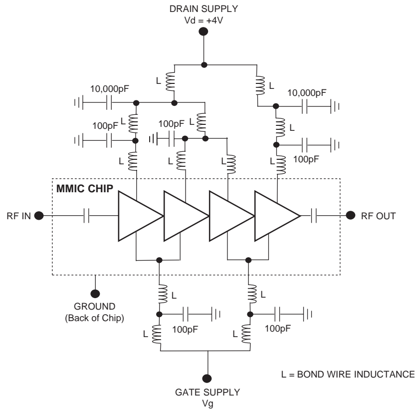
Figure 3. Recommended Application Schematic Circuit Diagram
