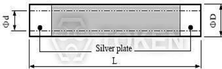
Tubular High Voltage Resistors (RMCD) Dimensions
