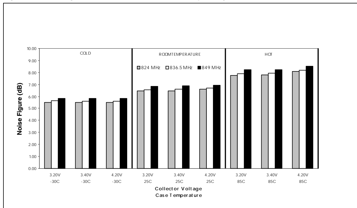
Figure 15. Noise Figure Variation Over Recommended Operating Conditions
