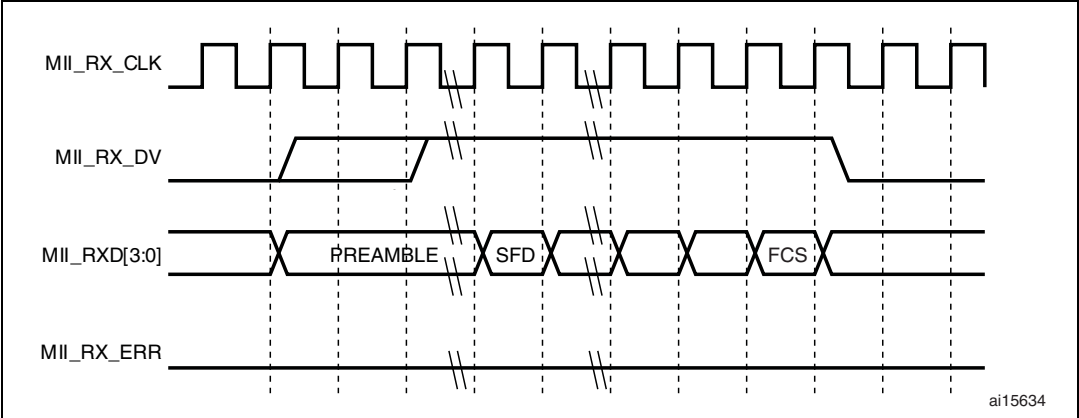
Figure 343. Reception with no error
