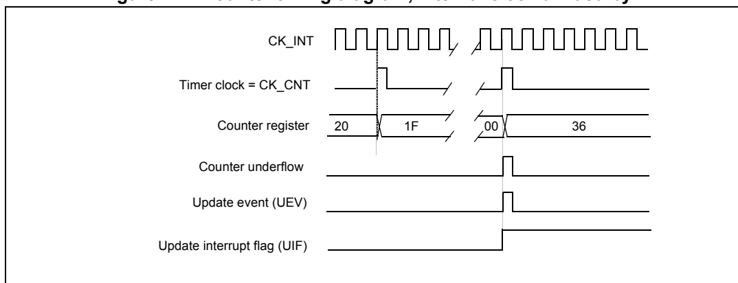
Figure 113. Counter timing diagram, Update event
