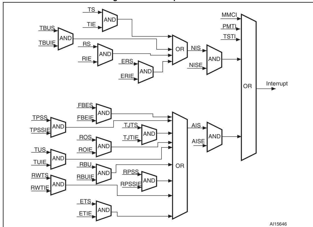
Figure 358. Interrupt scheme
