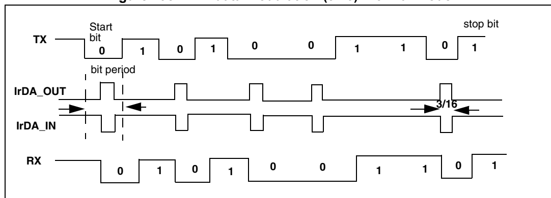
Figure 295. IrDA data modulation (3/16) -normal mode
