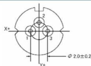
View from below, dimensions in mm
