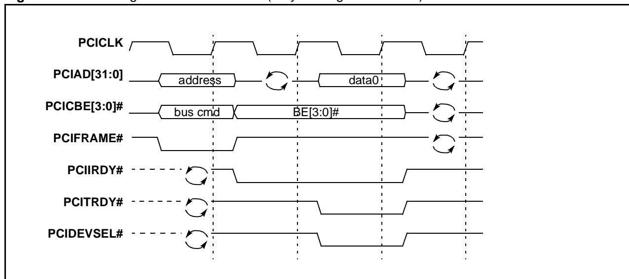
Figure 14. PCI Target read - Slave Read (1-cycle single word read)
