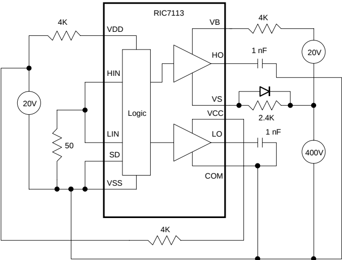
Figure 7. Static Bias Conditions for Total Ionizing DoseTest
