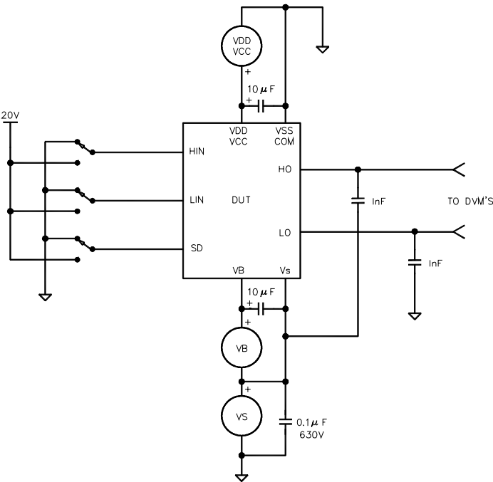
Figure 8. Static Bias Conditions for Single Event Effect Test
