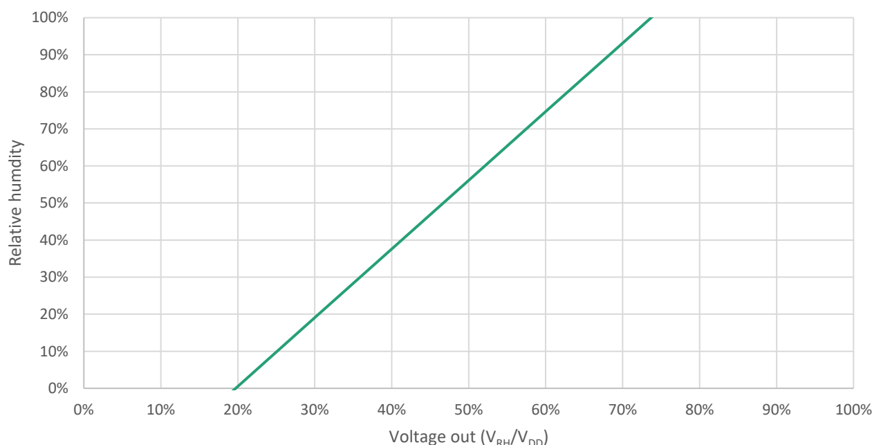
Figure 1: Relationship between the ratiometric analog voltage output and the measured relative humidity
