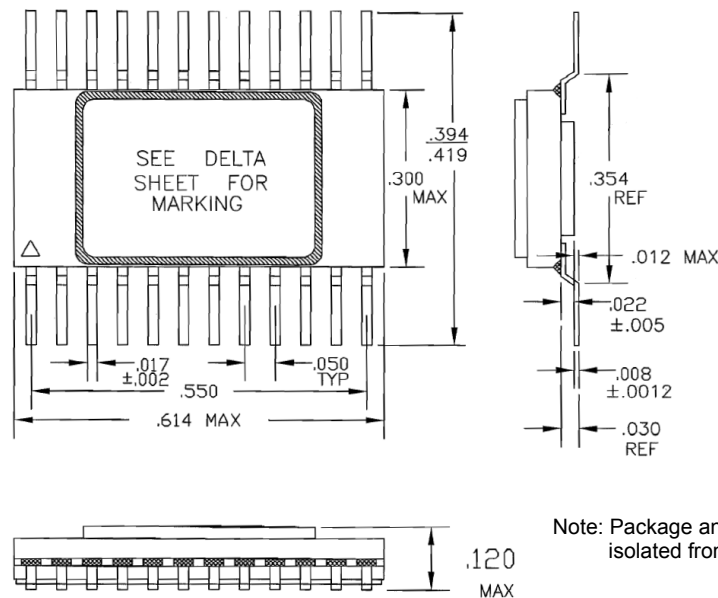
FIGURE 4: PACKAGE OUTLINE
