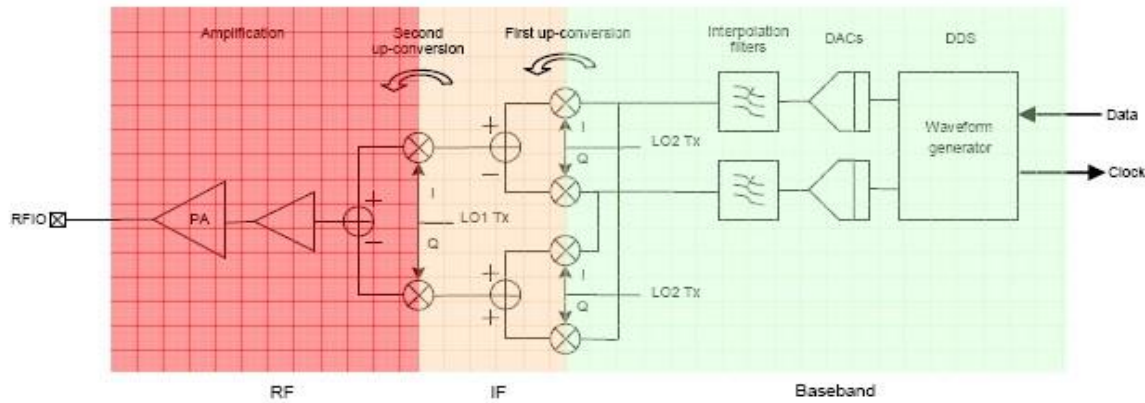
Figure 8: Transmitter Architecture
