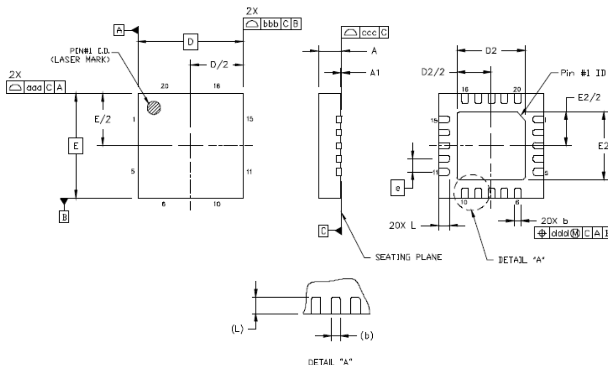
Figure 25. 20-Pin Quad Flat No-Lead (QFN)
