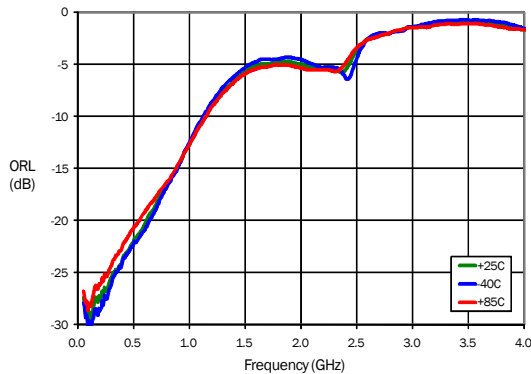
Output RL versus Temperature, Max Gain
