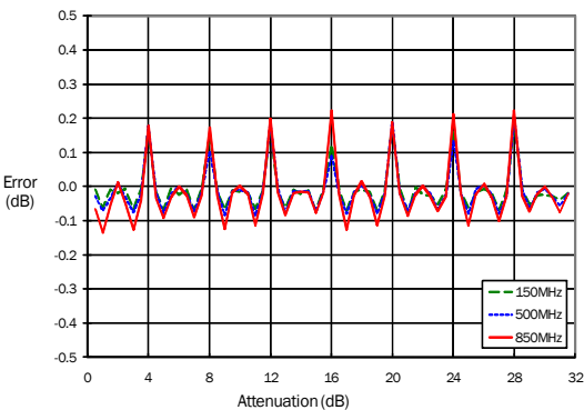
Successive Step Error versus Attenuation, 25C
