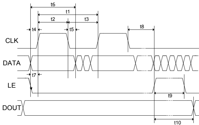
SPI Timing Diagram
