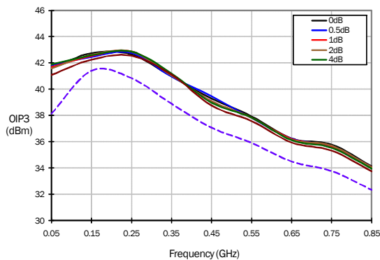
OIP3 versus Frequency, Max Gain
