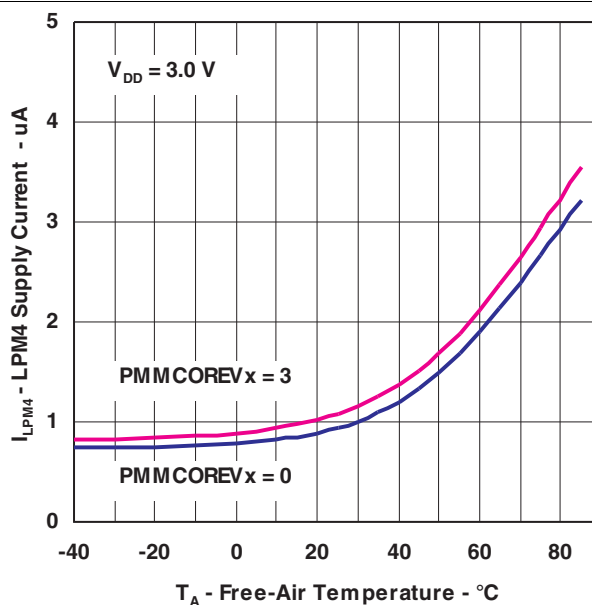
Figure 5-4. LPM4 Supply Current vs Temperature
