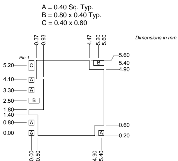
Metal Land Pattern
