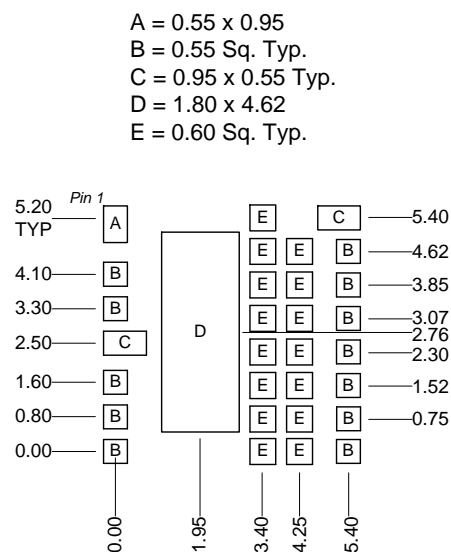
Solder Mask Pattern
