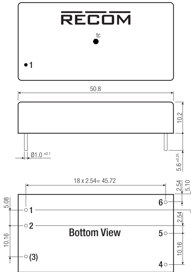
Dimension Drawing (mm)
