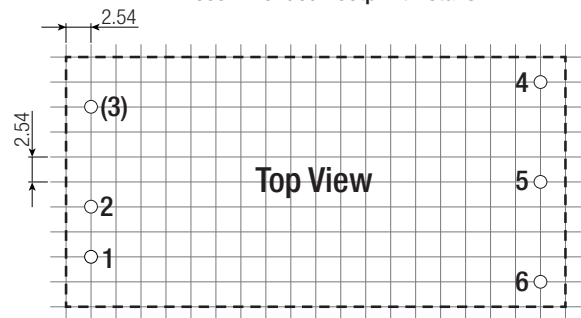
Recommended Footprint Details
