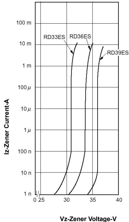
Figure 5. Zener current vs. zener voltage
