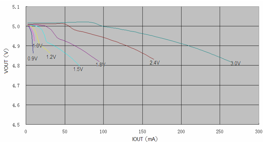
Figure6. Output Voltage VS Output current
