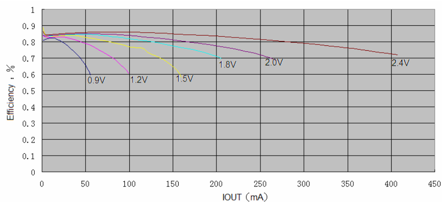
Figure3. Efficiency VS Output current
