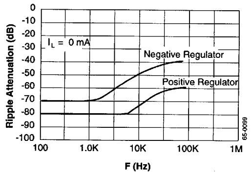
Figure 6. Ripple Rejection
