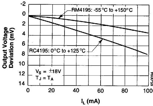
Figure 1. Output Load Regulation
