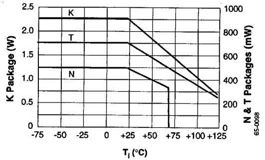
Figure 4. Power Dissipation
