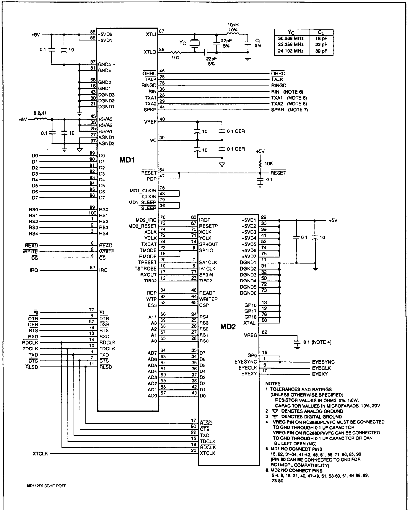
Figure 5. Typical interface to Modem In PQFPs
