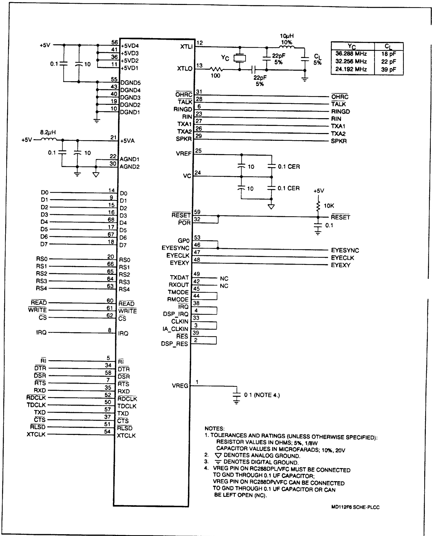
Figure 6. Typical Interface to Modem in PLCC
