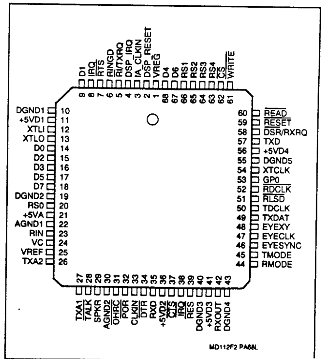
Figure 2. Pin Signals- 68-Pin PLCC
