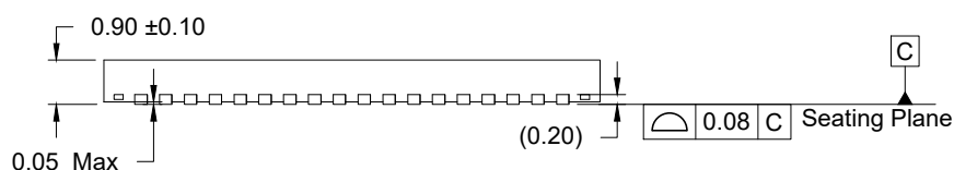
SIDE VIEW
