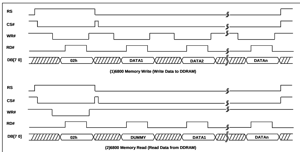
Figure 6-31 : 6800 Memory Write/Memory Read
