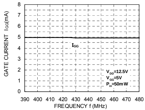
GATE CURRENT versus FREQUENCY
