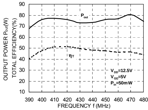
OUTPUT POWER, TOTAL EFFICIENCY, versus FREQUENCY
