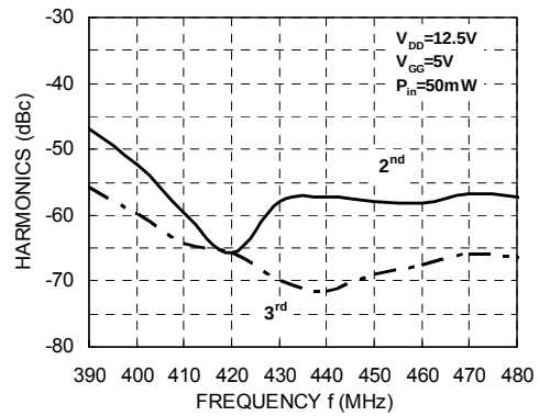
2 nd , 3 rd HARMONICS versus FREQUENCY
