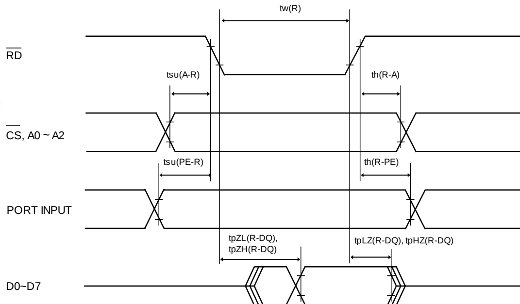
Read operation
