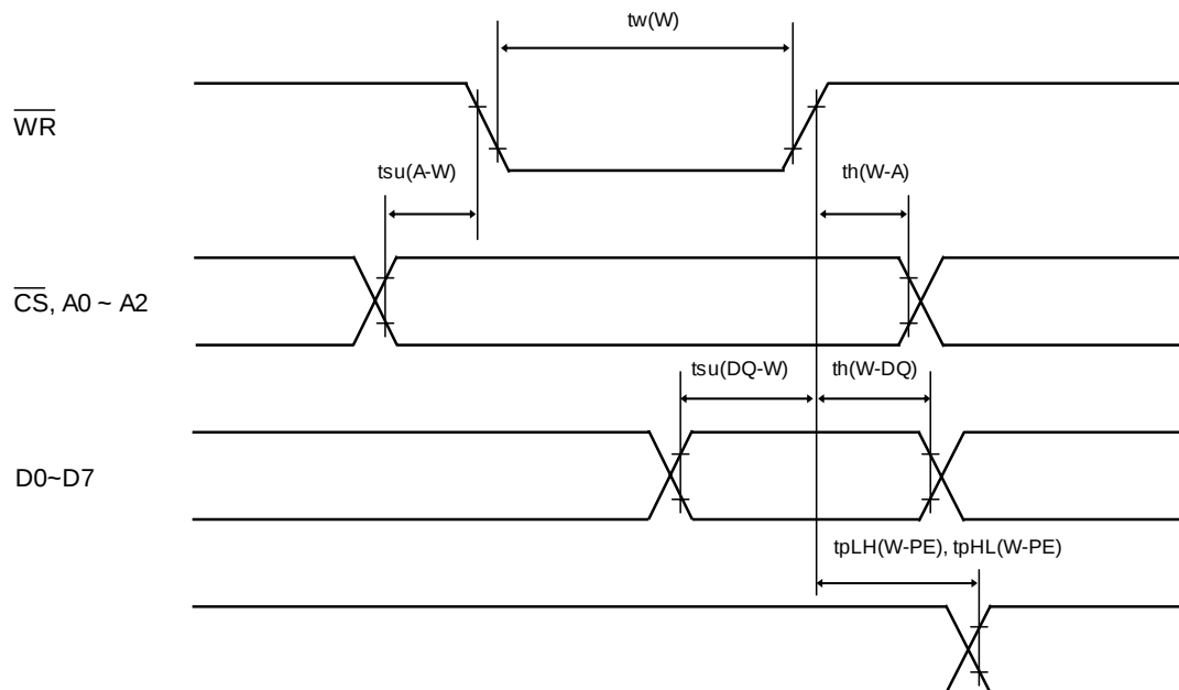
Write operation
