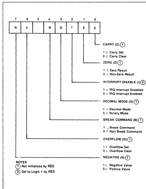
Figure 3-6. Processor Status Register
