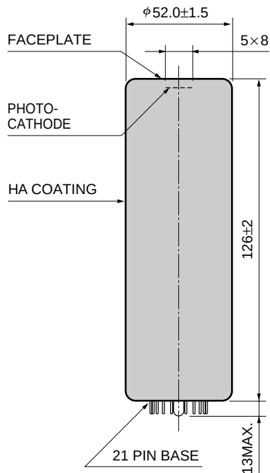
Figure 3: Dimensional Outline and Basing Diagram (Unit: mm)
