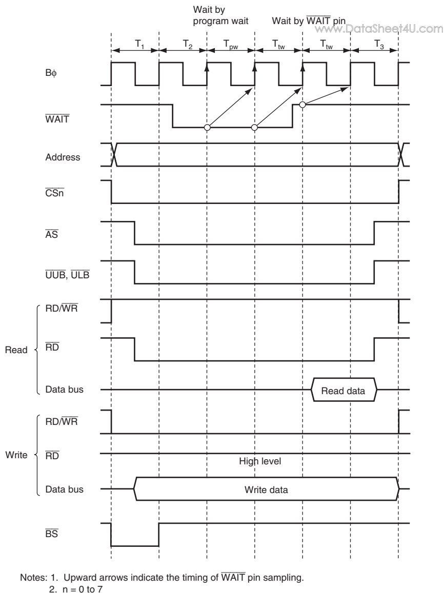
Figure 6.25 Example of Wait Cycle Insertion Timing
