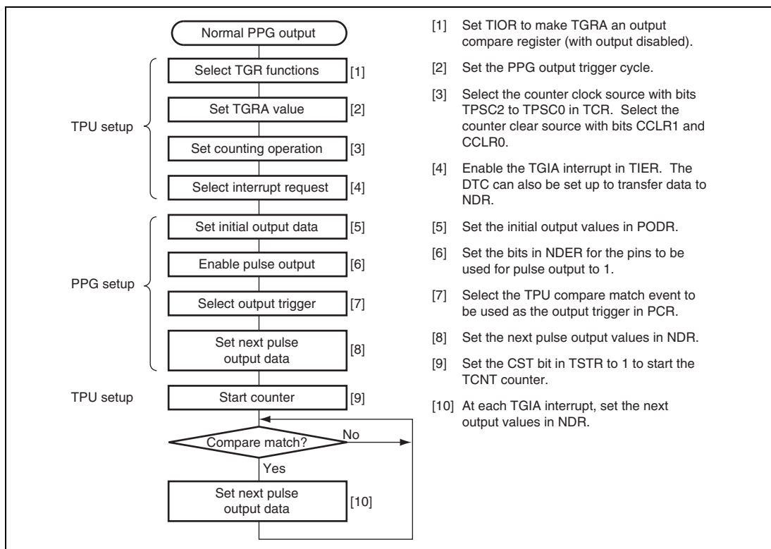
Figure 10.4 Setup Procedure for Normal Pulse Output (Example)
