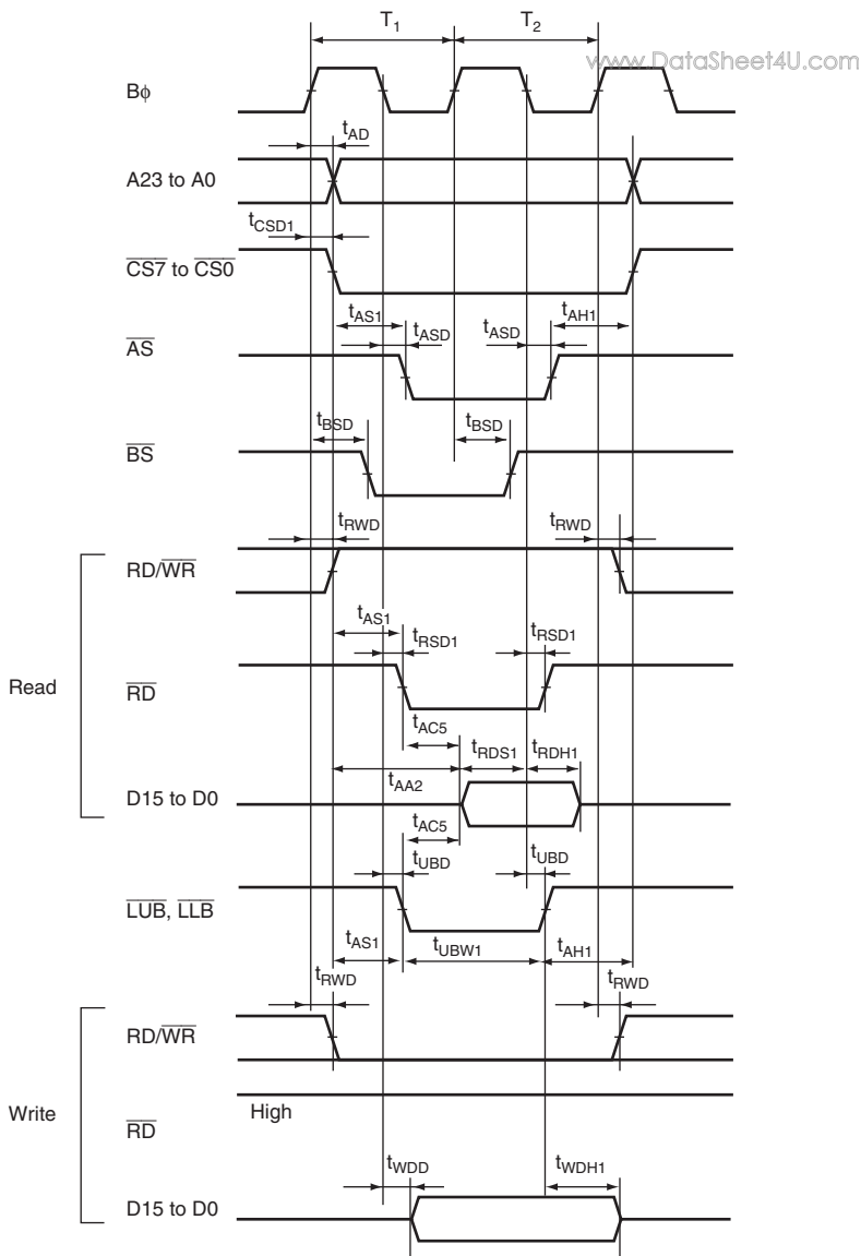
Figure 20.13 Byte Control SRAM: 2-State Read/Write Access
