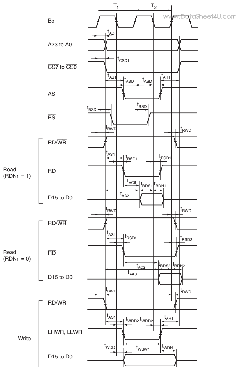
Figure 20.8 Basic Bus Timing: 2-State Access
