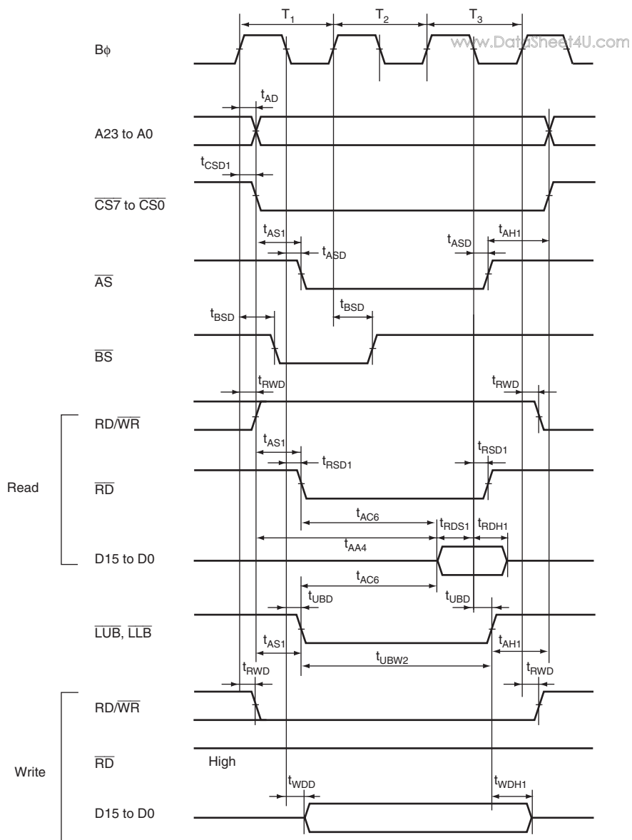
Figure 20.14 Byte Control SRAM: 3-State Read/Write Access
