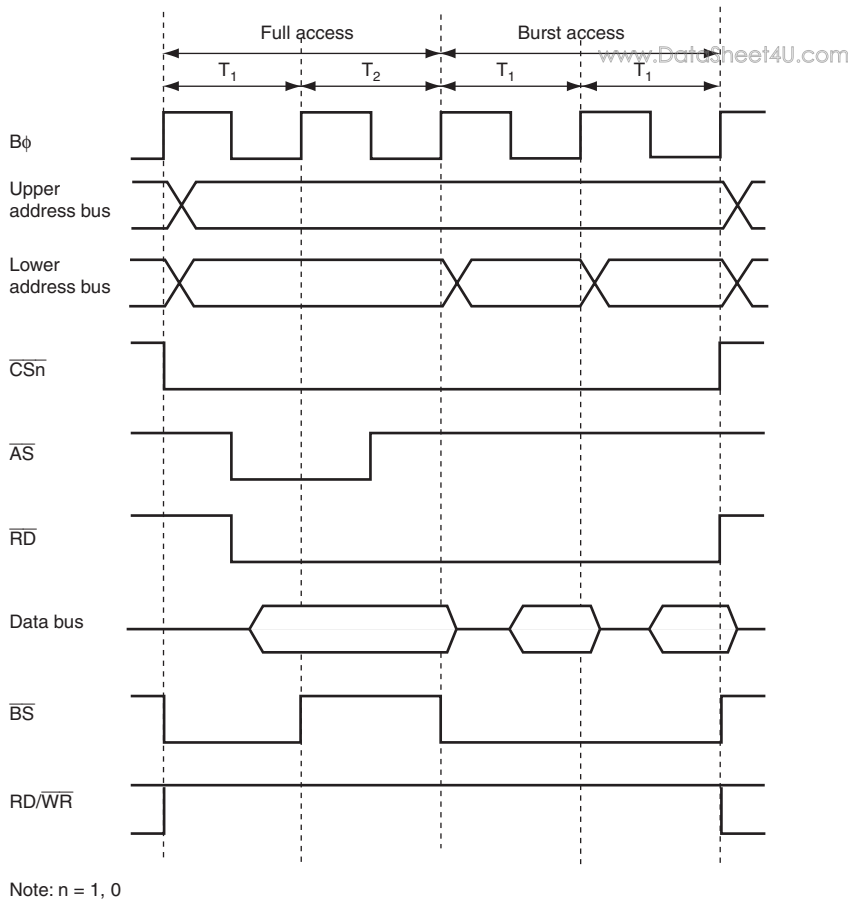
Figure 6.27 Example of Burst ROM Access Timing ( AST_n = 0 , One Burst Cycle)
