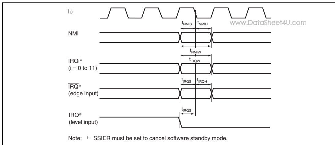
Figure 20.7 Interrupt Input Timing
