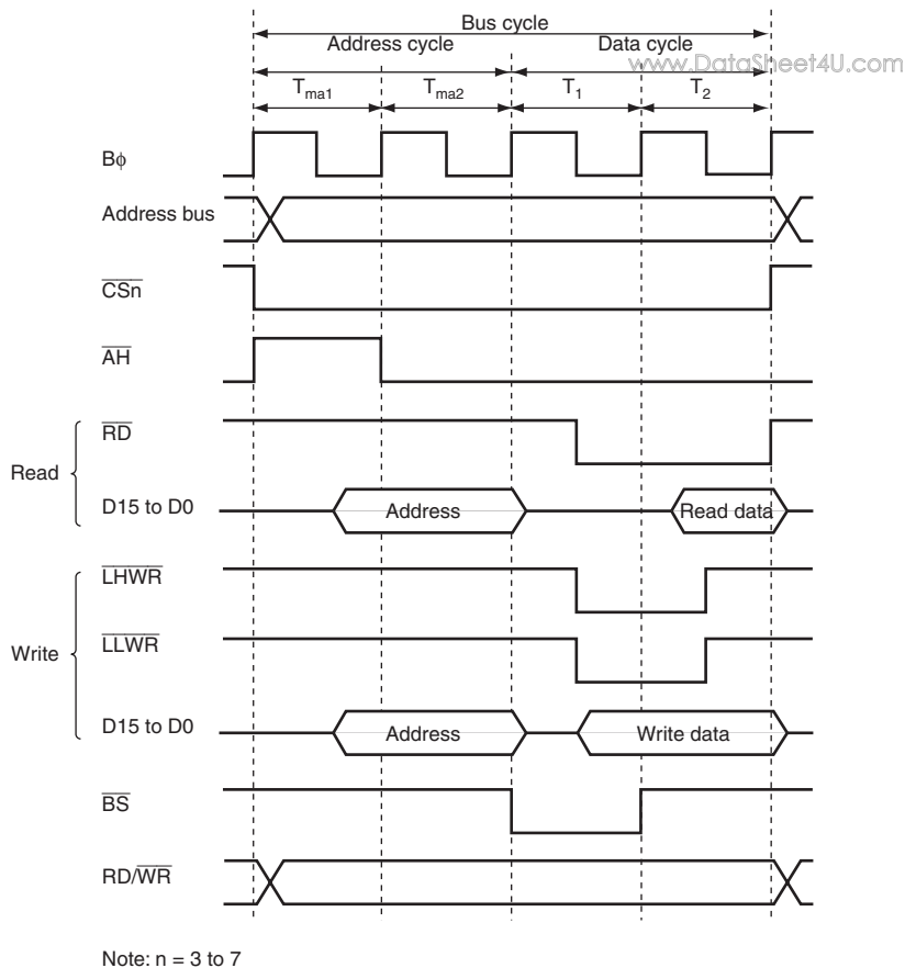
Figure 6.29 16-Bit Access Space Access Timing (ABWHn = 0, ABWLn = 1)
