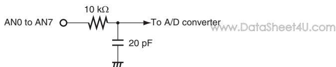
Figure 14.10 Analog Input Pin Equivalent Circuit
