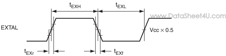
Figure 20.5 External Input Clock Timing
