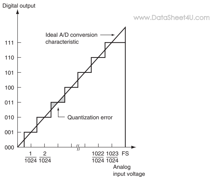
Figure 14.6 A/D Conversion Accuracy Definitions
