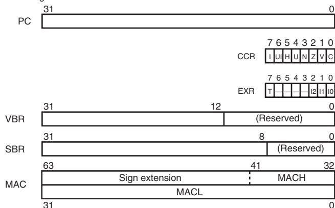
Control Registers
