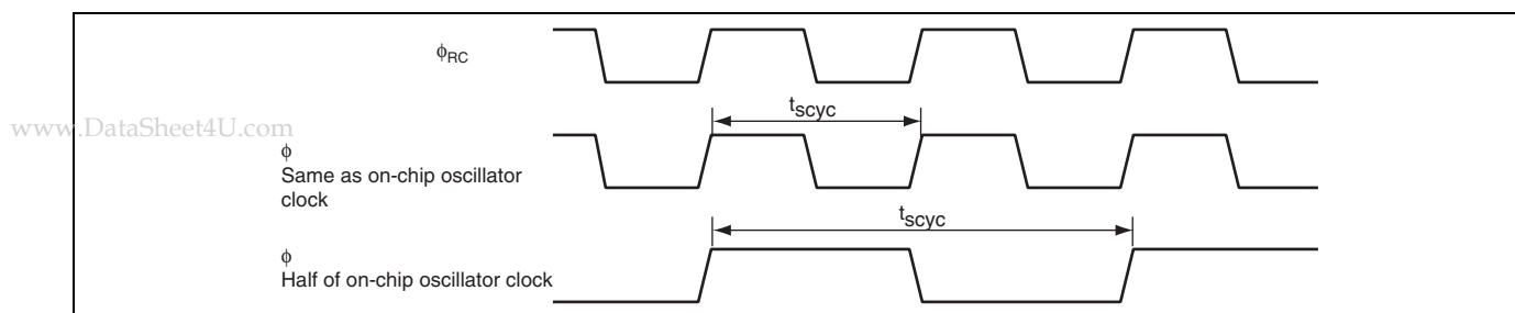
Figure 4.2 System Clock Timing (Internal clock)
