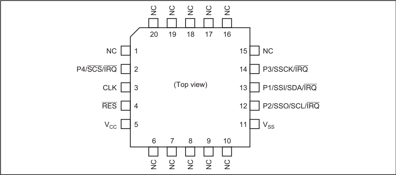
Figure 2 Pin Assignment
