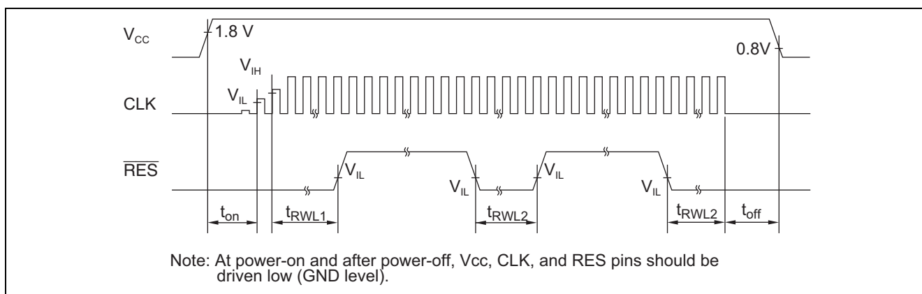
Figure 6 Power ON/OFF and \overline{\text{RES}} Input Timing
