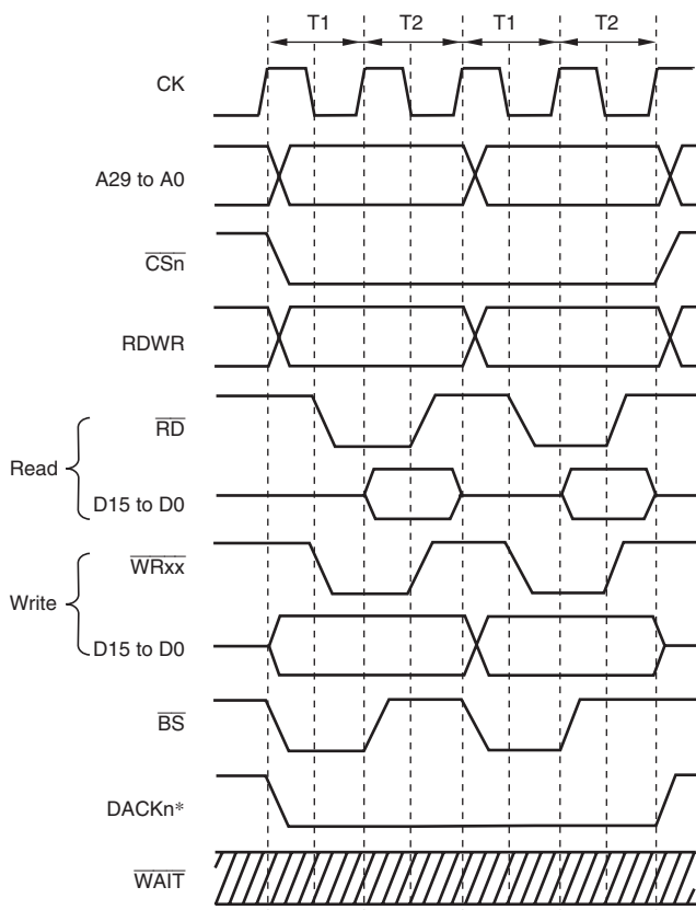
Figure 9.4 Continuous Access for Normal Space 2 Bus Width = 16 Bits, Longword Access, WM Bit in \overline{CSnWCR} = 1 (Access Wait = 0, Cycle Wait = 0)
