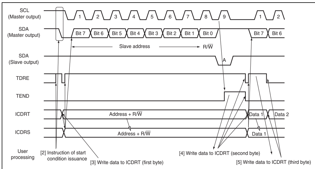
Figure 18.5 Master Transmit Mode Operation Timing (1)
