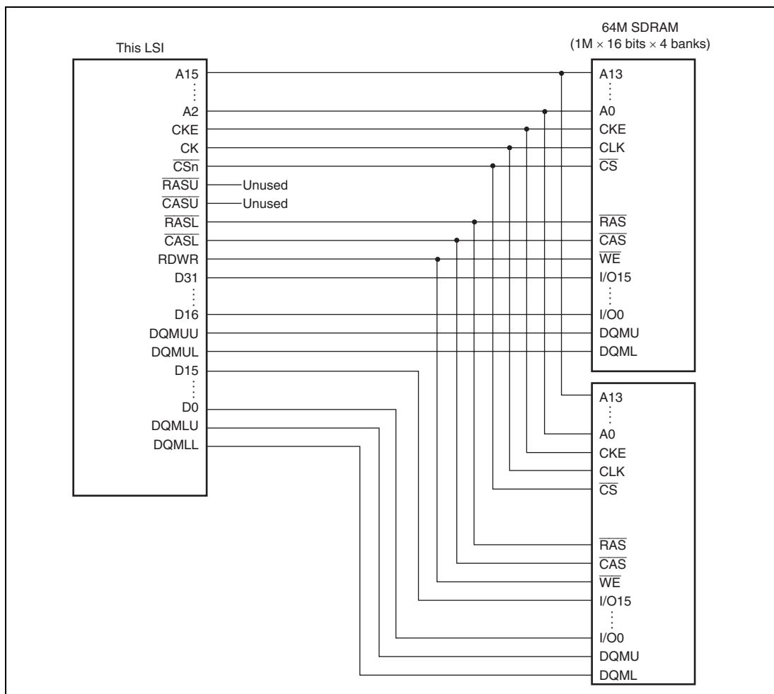
Figure 9.14 Example of 32-Bit Data Width SDRAM Connection (RASU and CASU are not Used)
