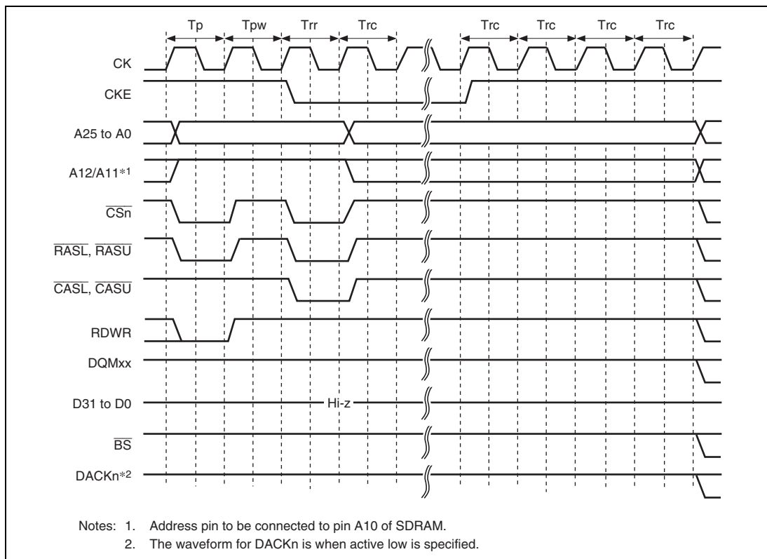
Figure 9.29 Self-Refresh Timing
