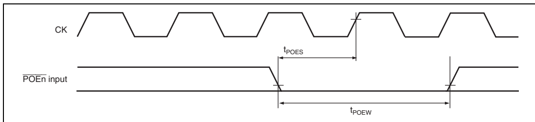
Figure 28.59 POE Input Timing
