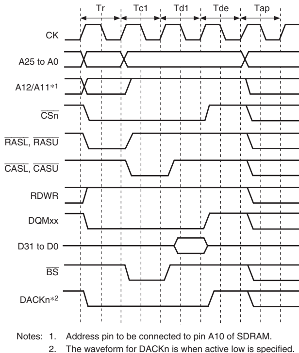
Figure 9.19 Single Read Basic Timing (Auto-Precharge)
