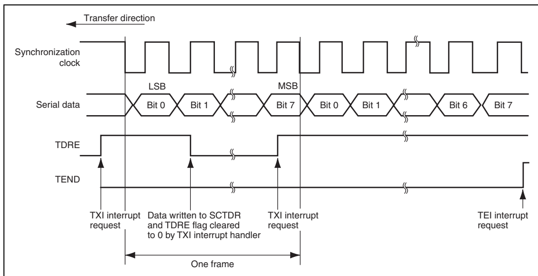
Figure 15.11 Example of SCI Transmit Operation
