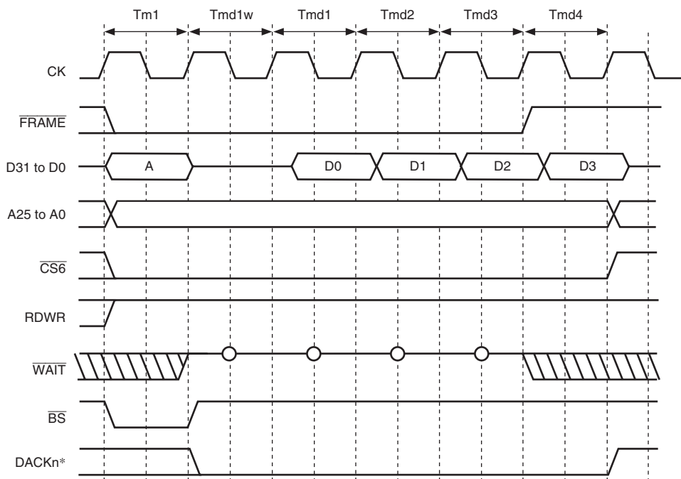
Figure 9.46 Burst MPX Space Access Timing (Burst Read, No Wait or Software Wait 1)
