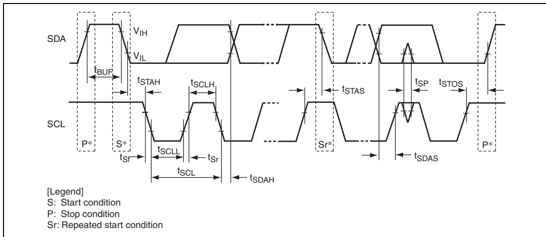
Figure 28.60 I²C2 Input/Output Timing
