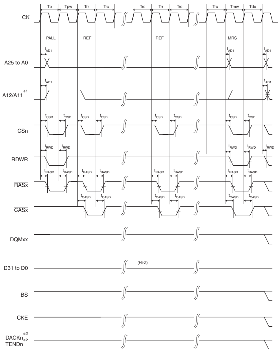
Figure 28.40 Synchronous DRAM Mode Register Write Timing (WTRP = 1 Cycle)
