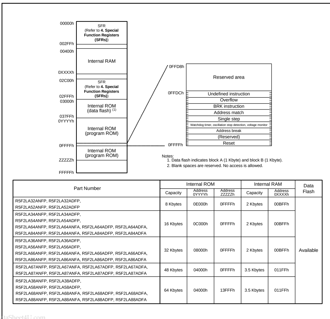
Figure 3.1 Memory Map
