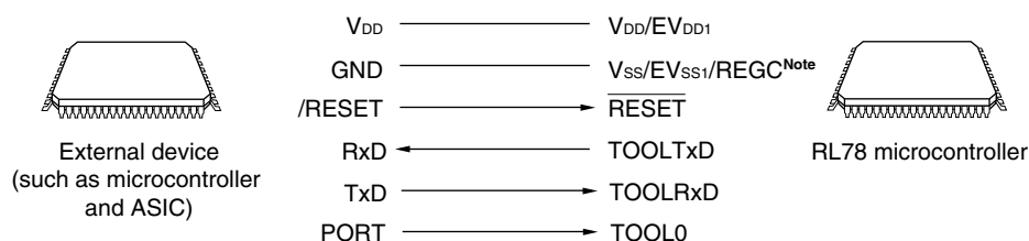
Figure 33-4. Communication with External Device
