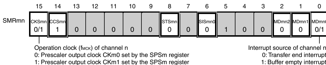
Figure 18-63. Example of Contents of Registers for Slave Transmission/Reception of 3-Wire Serial I/O (CSI00) (1/2)
