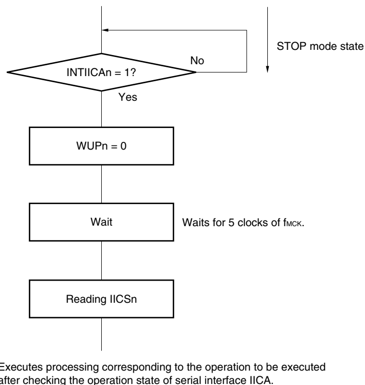
<R> Figure 19-23. Flow When Setting WUPn = 0 upon Address Match (Including Extension Code Reception)
