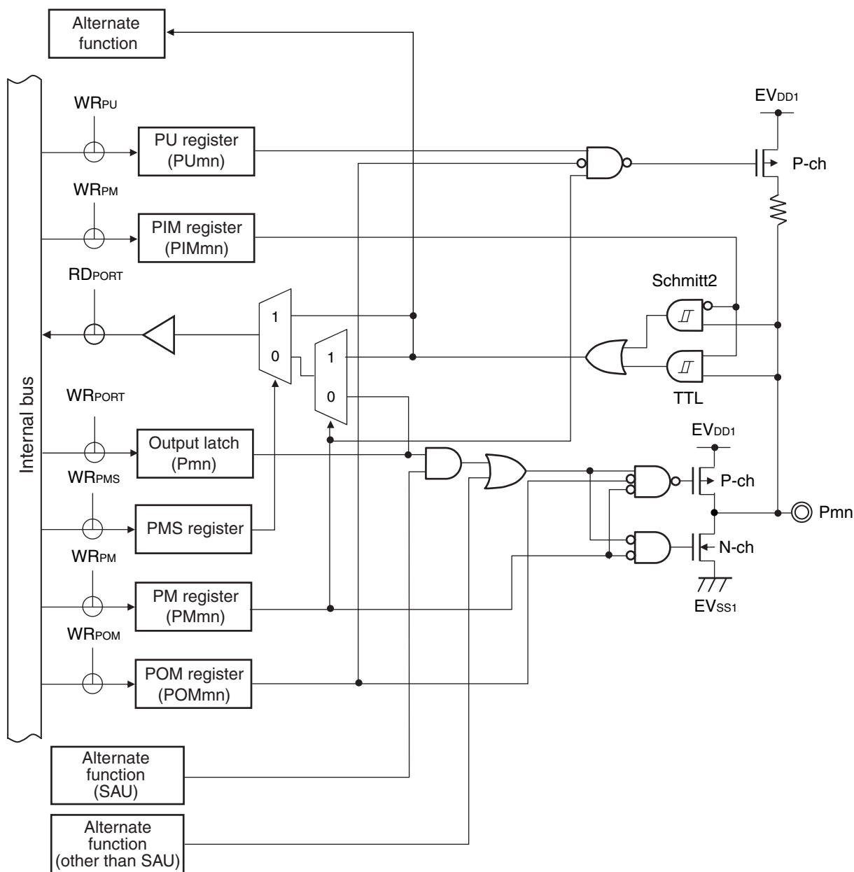
Figure 2-14. Pin Block Diagram for Pin Type 8-1-4
