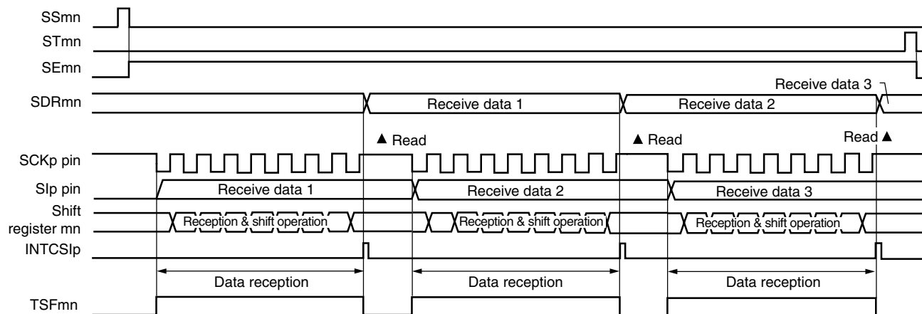
Figure 18-61. Timing Chart of Slave Reception (in Single-reception Mode)
