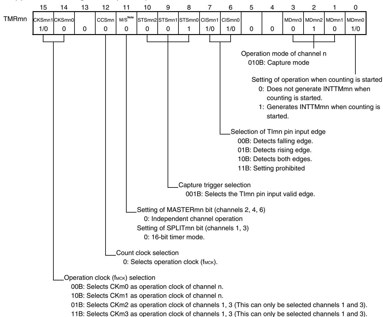
Figure 7-52. Example of Set Contents of Registers to Measure Input Pulse Interval
