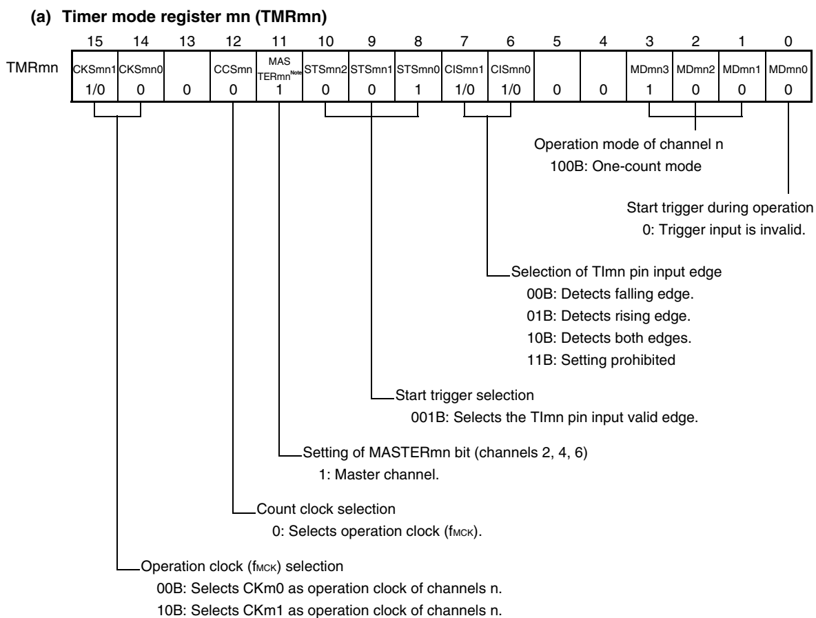
&lt;R&gt; Figure 7-64. Example of Set Contents of Registers When One-Shot Pulse Output Function Is Used (Master Channel)
