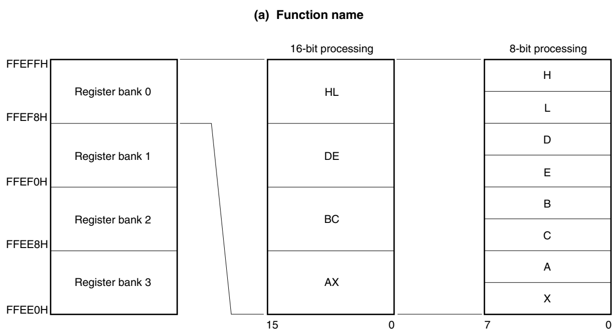
Figure 3-8. Configuration of General-Purpose Registers
