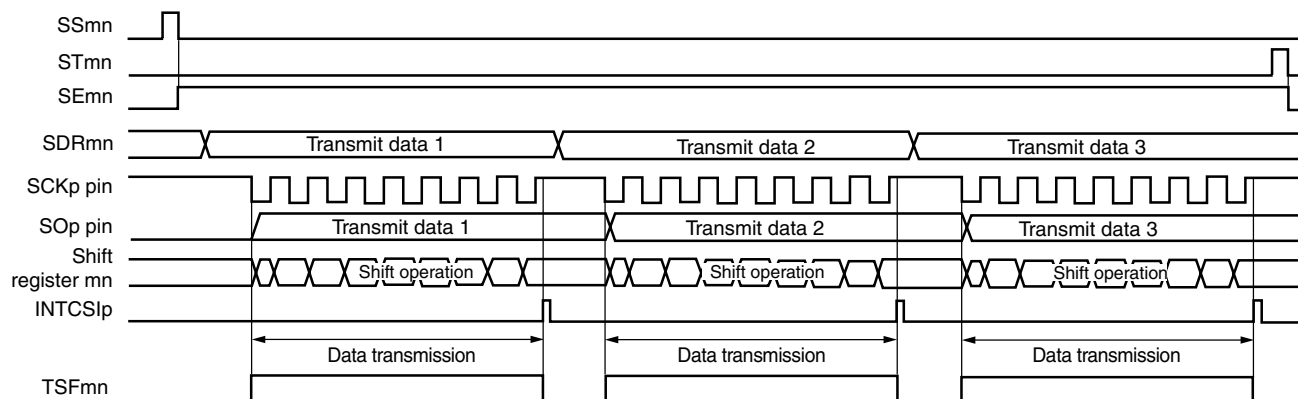
Figure 18-53. Timing Chart of Slave Transmission (in Single-Transmission Mode)
