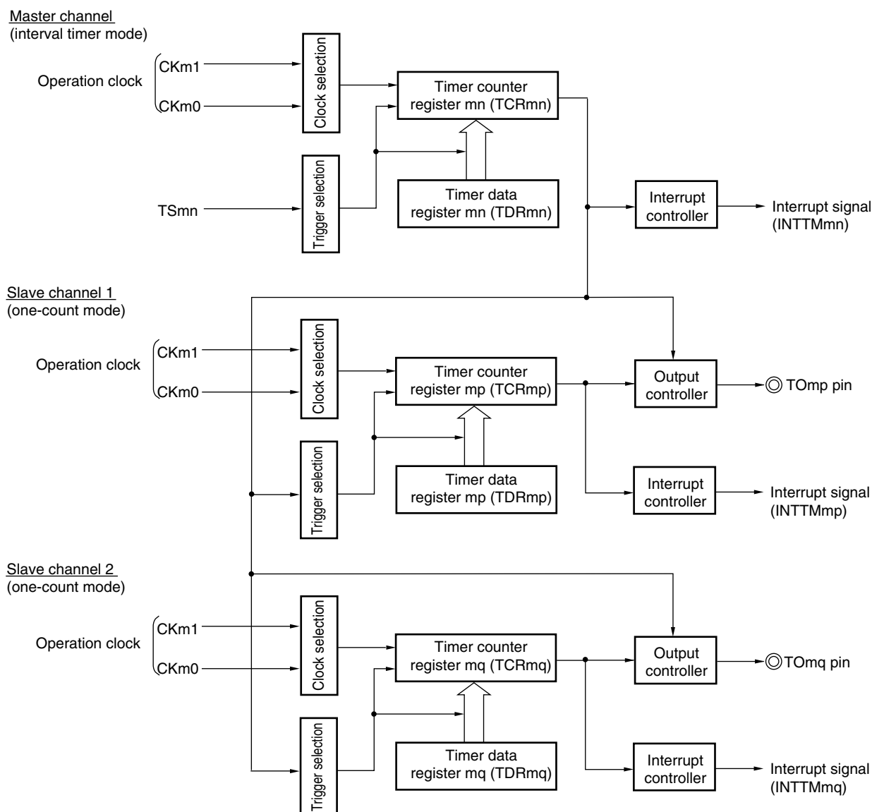
Figure 7-72. Block Diagram of Operation as Multiple PWM Output Function (Output Two Types of PWMs)
