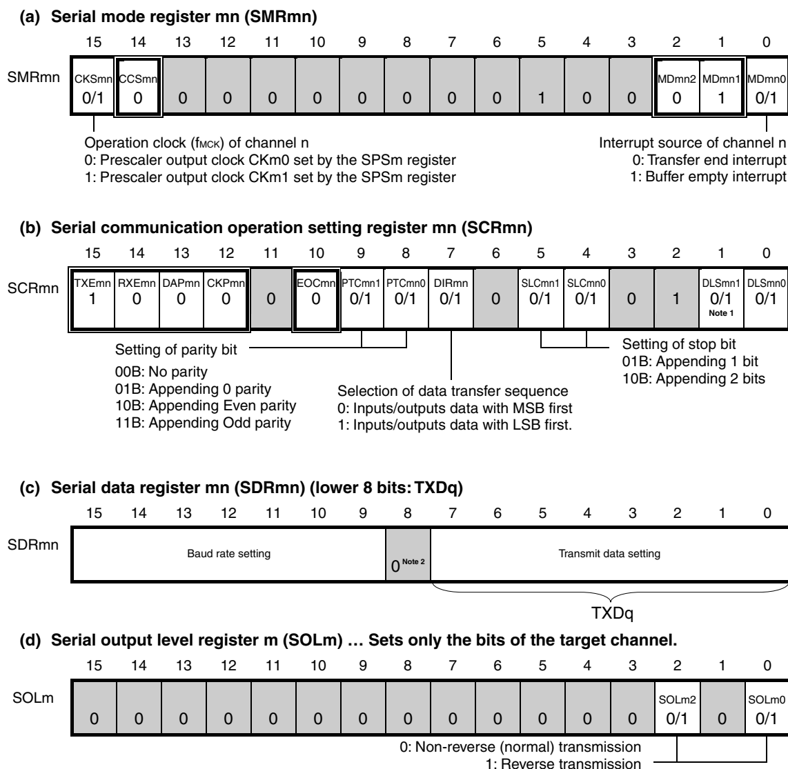
Figure 18-76. Example of Contents of Registers for UART Transmission of UART (UART0 to UART2) (1/2)
