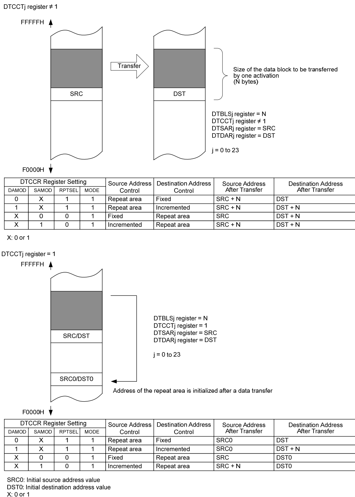
Figure 22-17. Data Transfers in Repeat Mode
