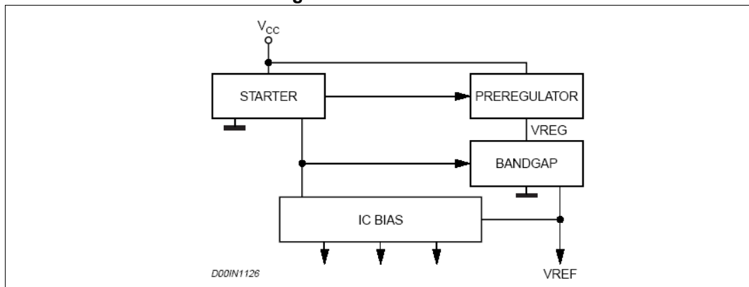
Figure 3. Internal circuit
