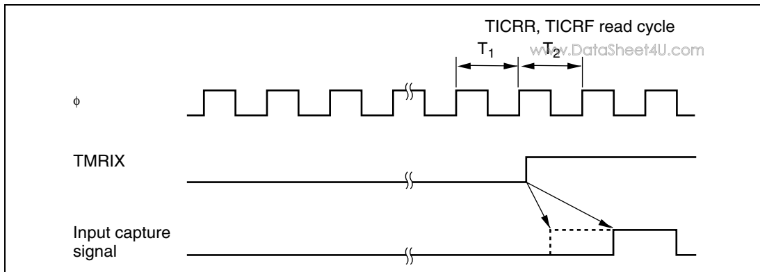
Figure 12.12 Timing of Input Capture Signal (Input capture signal is input during TICRR and TCRF read)
