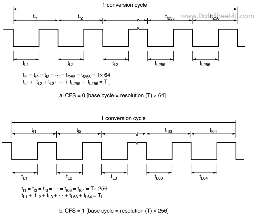
Figure 9.4 Output Waveform (OS = 0, DADR corresponds to T_L )
