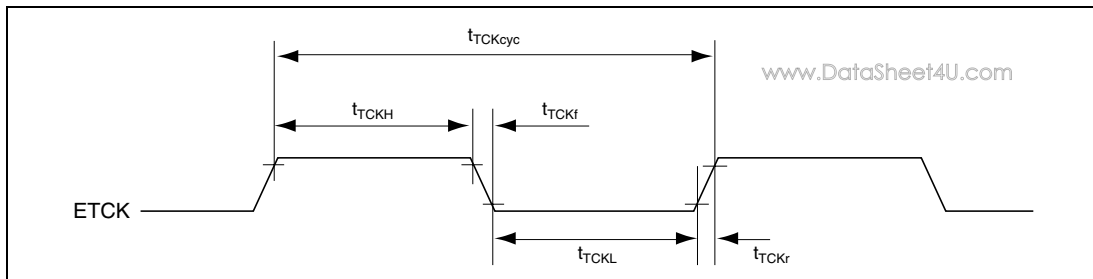
Figure 22.23 JTAG ECK Timing
