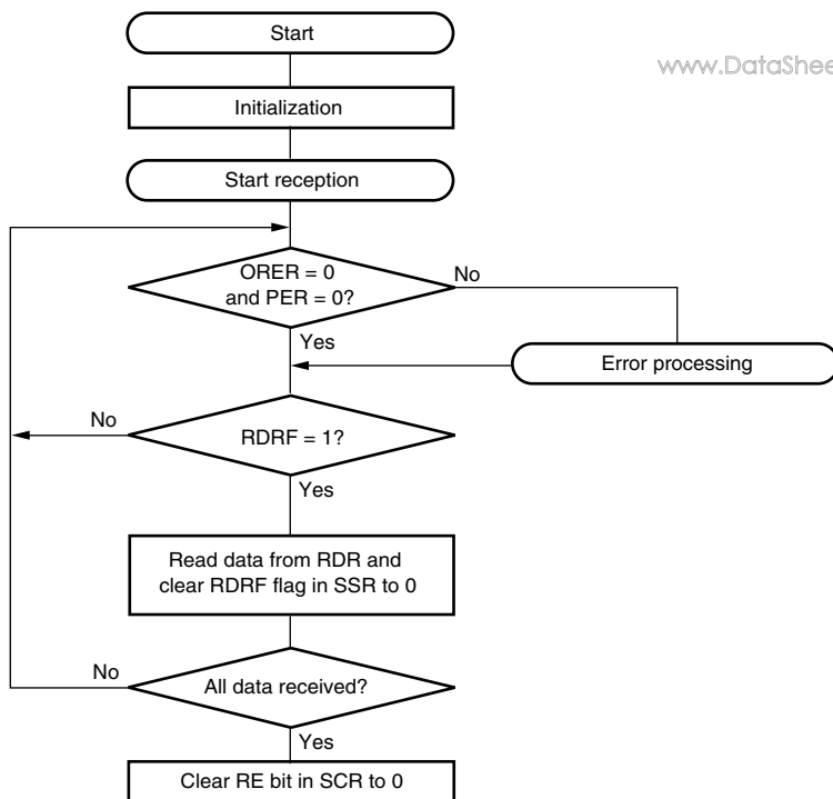
Figure 14.30 Sample Reception Flowchart
