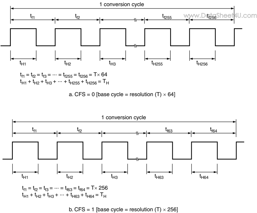
Figure 9.5 Output Waveform (OS = 1, DADR corresponds to TH)
