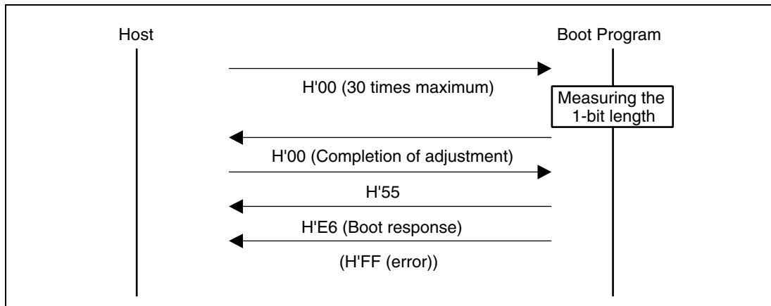
Figure 18.20 Bit-Rate-Adjustment Sequence
