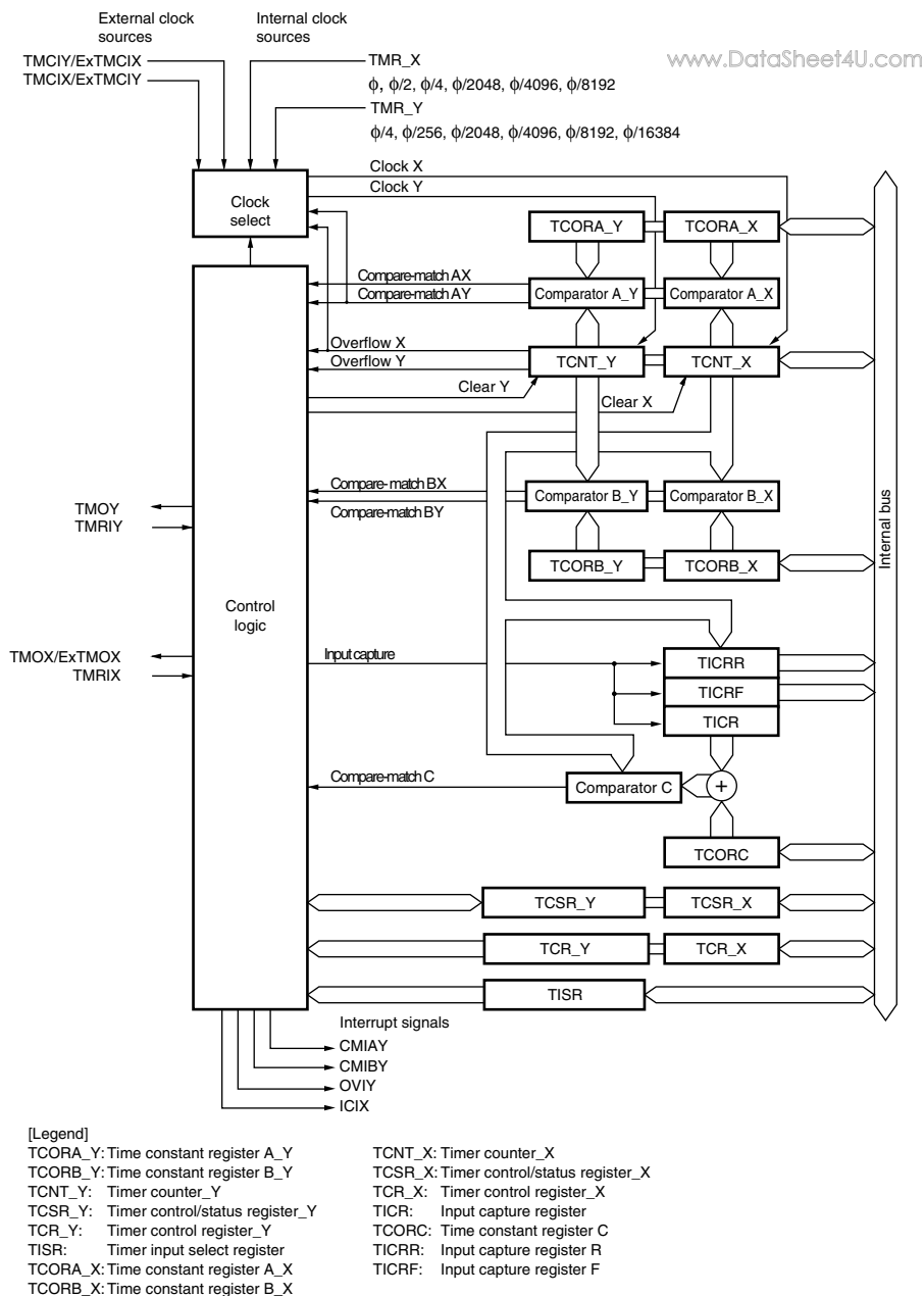
Figure 12.2 Block Diagram of 8-Bit Timer (TMR_Y and TMR_X)
