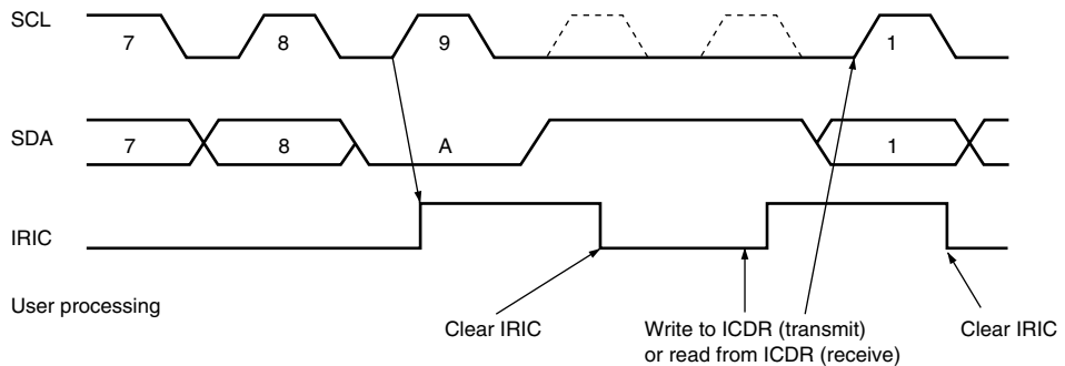
Figure 15.25 IRIC Setting Timing and SCL Control (1)
