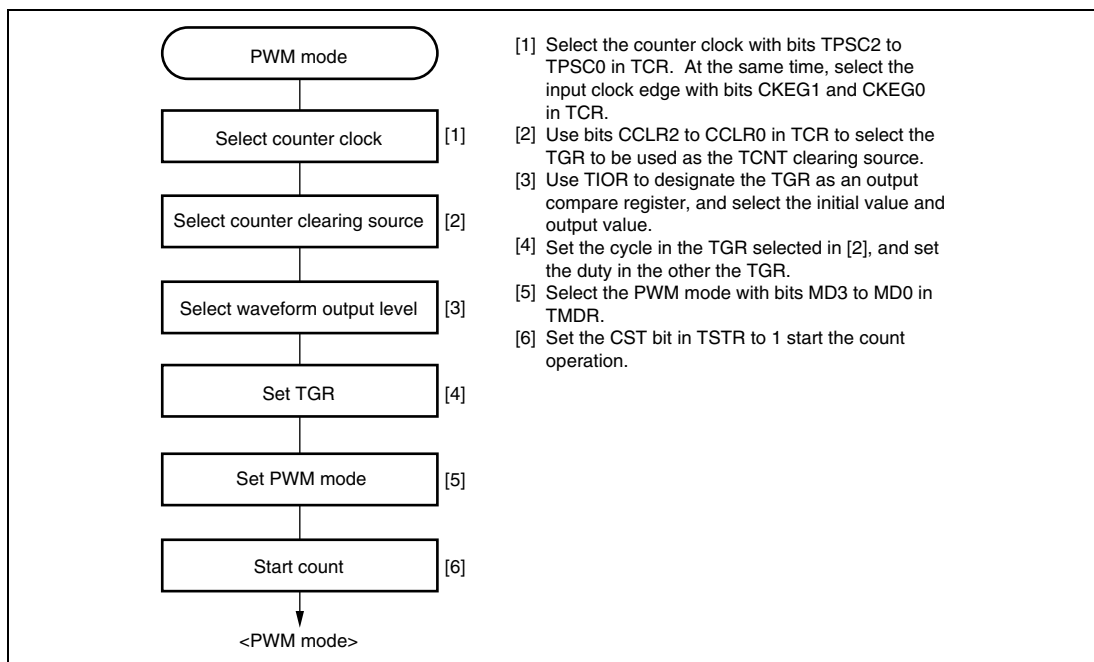
Figure 11.21 Example of PWM Mode Setting Procedure
