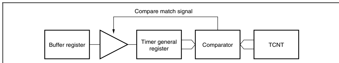
Figure 11.16 Compare Match Buffer Operation
