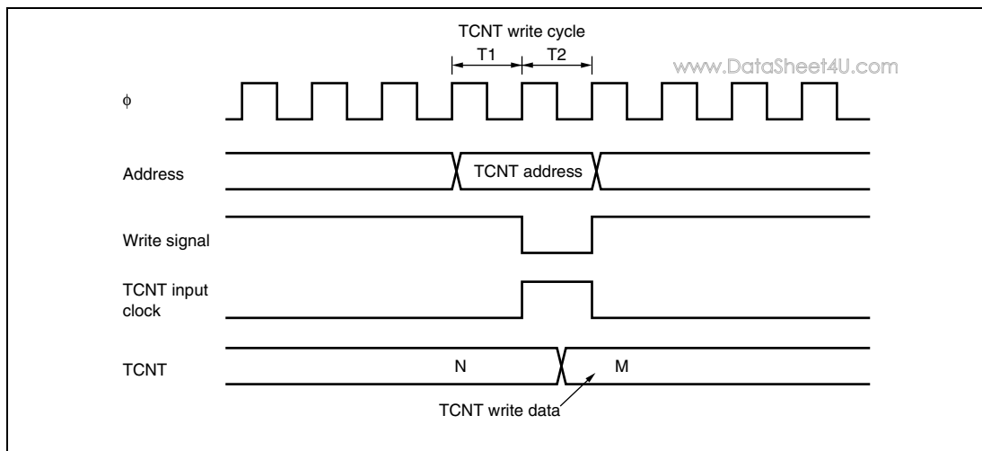
Figure 11.45 Conflict between TCNT Write and Increment Operations
