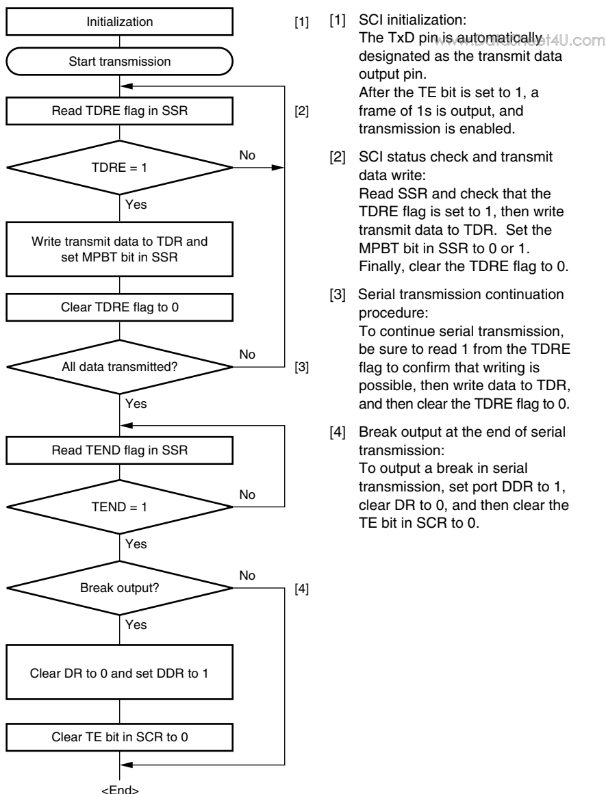
Figure 14.11 Sample Multiprocessor Serial Transmission Flowchart
