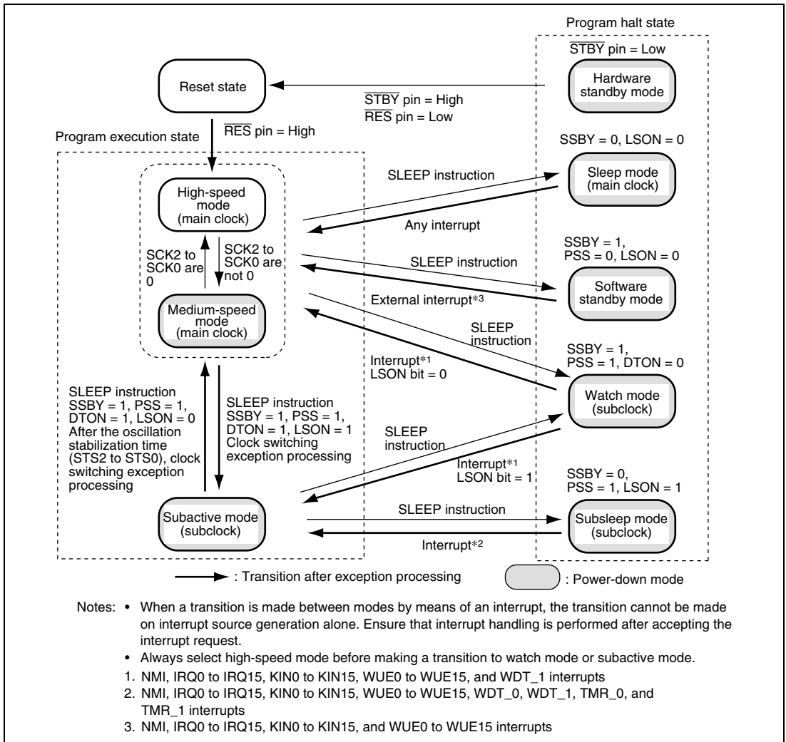
Figure 20.1 Mode Transition Diagram
