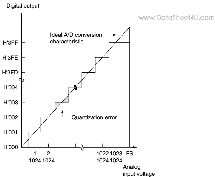
Figure 16.4 A/D Conversion Accuracy Definitions
