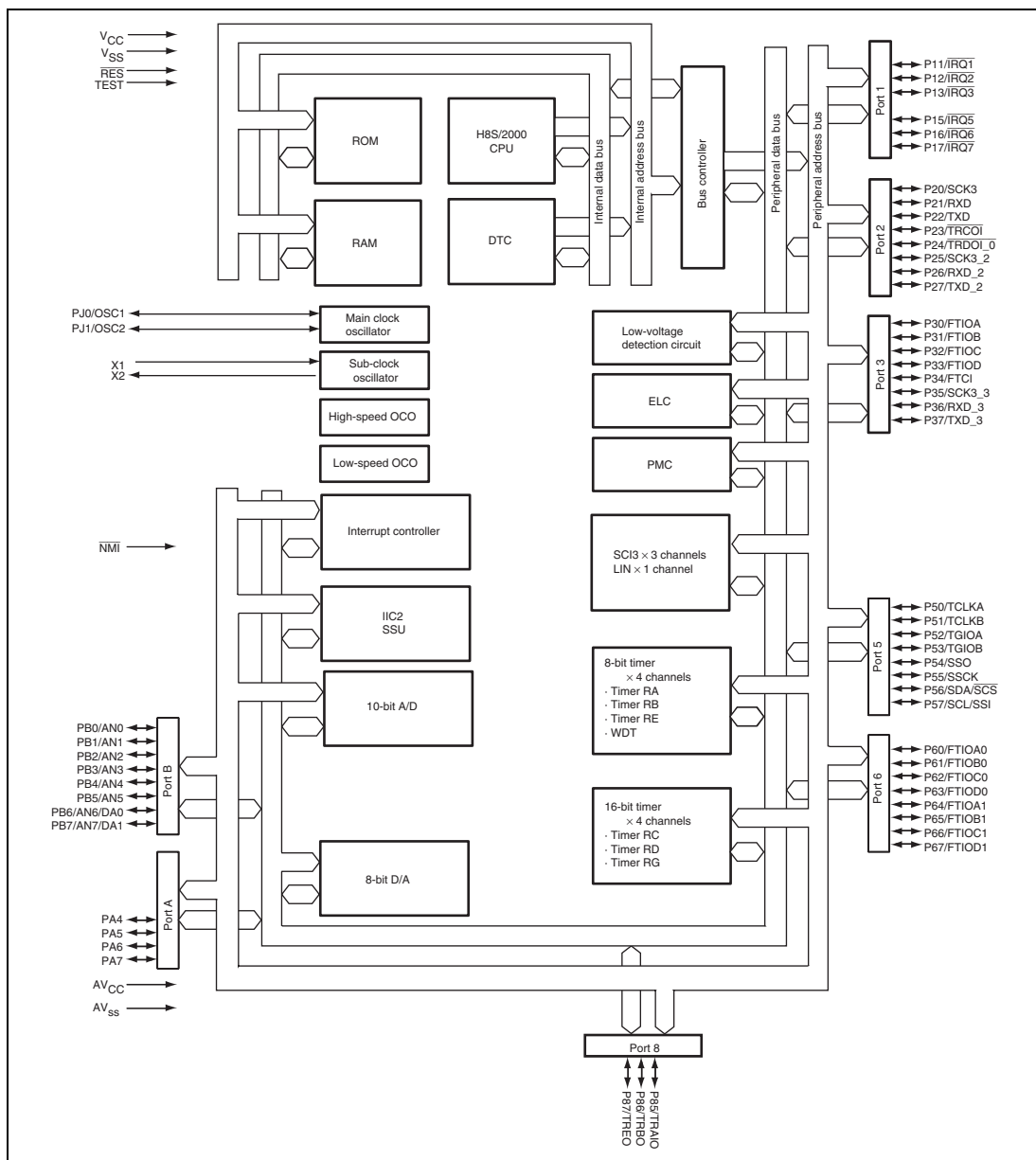
Figure 1.2 Block Diagram of H8S/20103 Group
