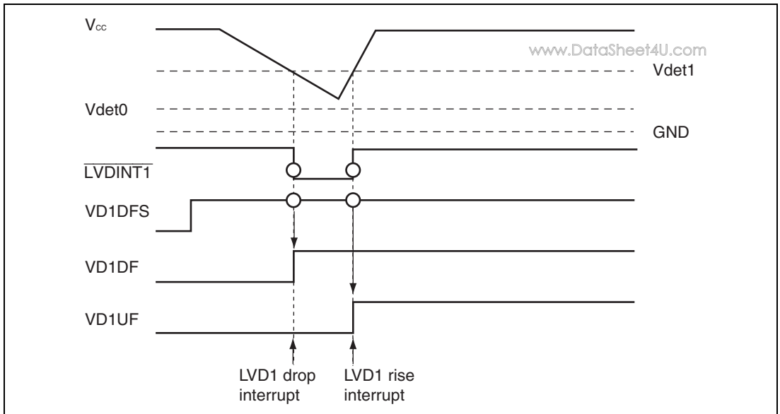
Figure 26.12 Operational Timing of LVDI1
