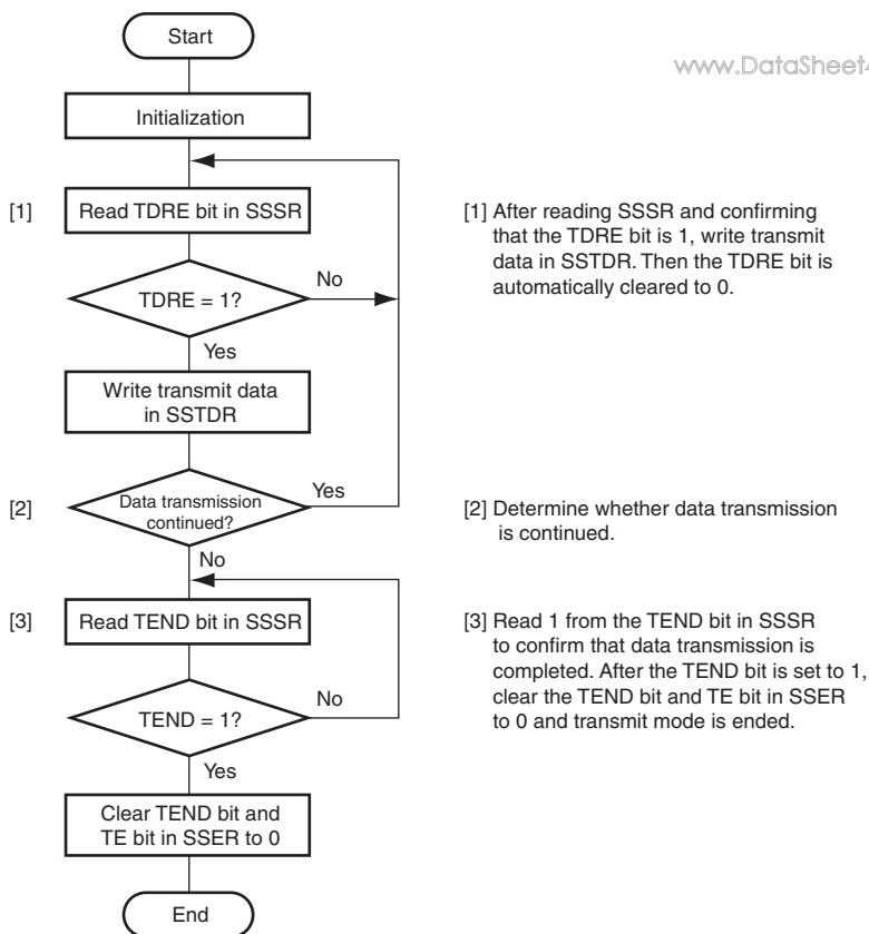
Figure 22.6 Sample Serial Transmission Flowchart
