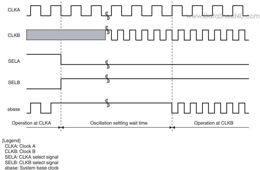
Figure 5.8 Timing of Clock Source Switching (When the switching destination clock source is stopped)
