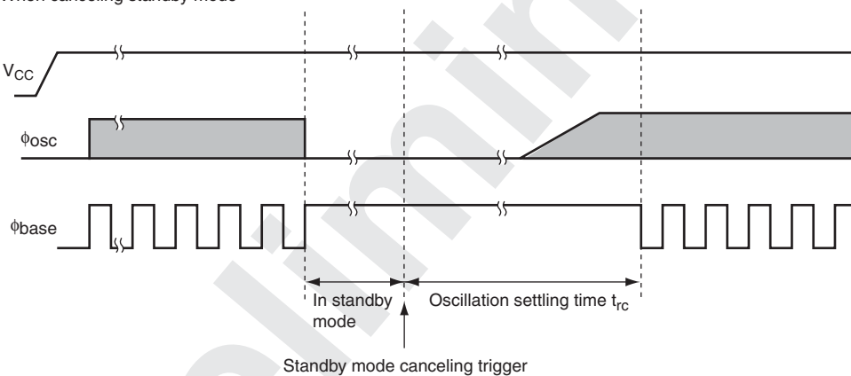
Figure 28.3 Timing of Oscillation Settling Time
