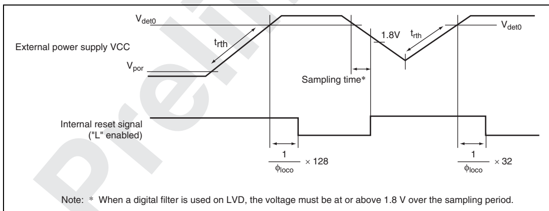
Figure 28.13 Timing of Power-On Reset
