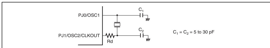
Figure 5.18 Example of Connection to Ceramic Resonator
