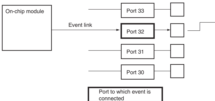
Figure 12.3 Event Linkage related to Single-Ports
