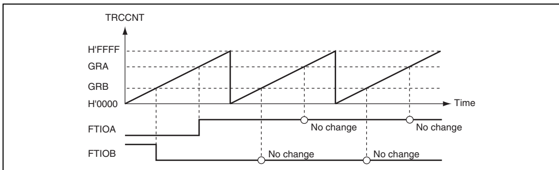
Figure 15.4 0 and 1 Output Example (TOA = 0, TOB = 1)
