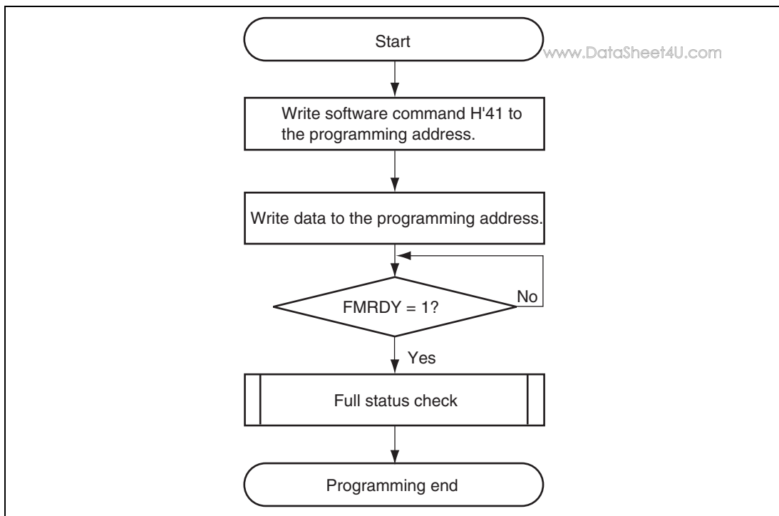
Figure 7.16 Programming Flowchart
