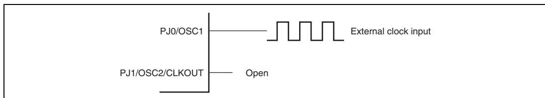
Figure 5.19 Example of External Clock Input
