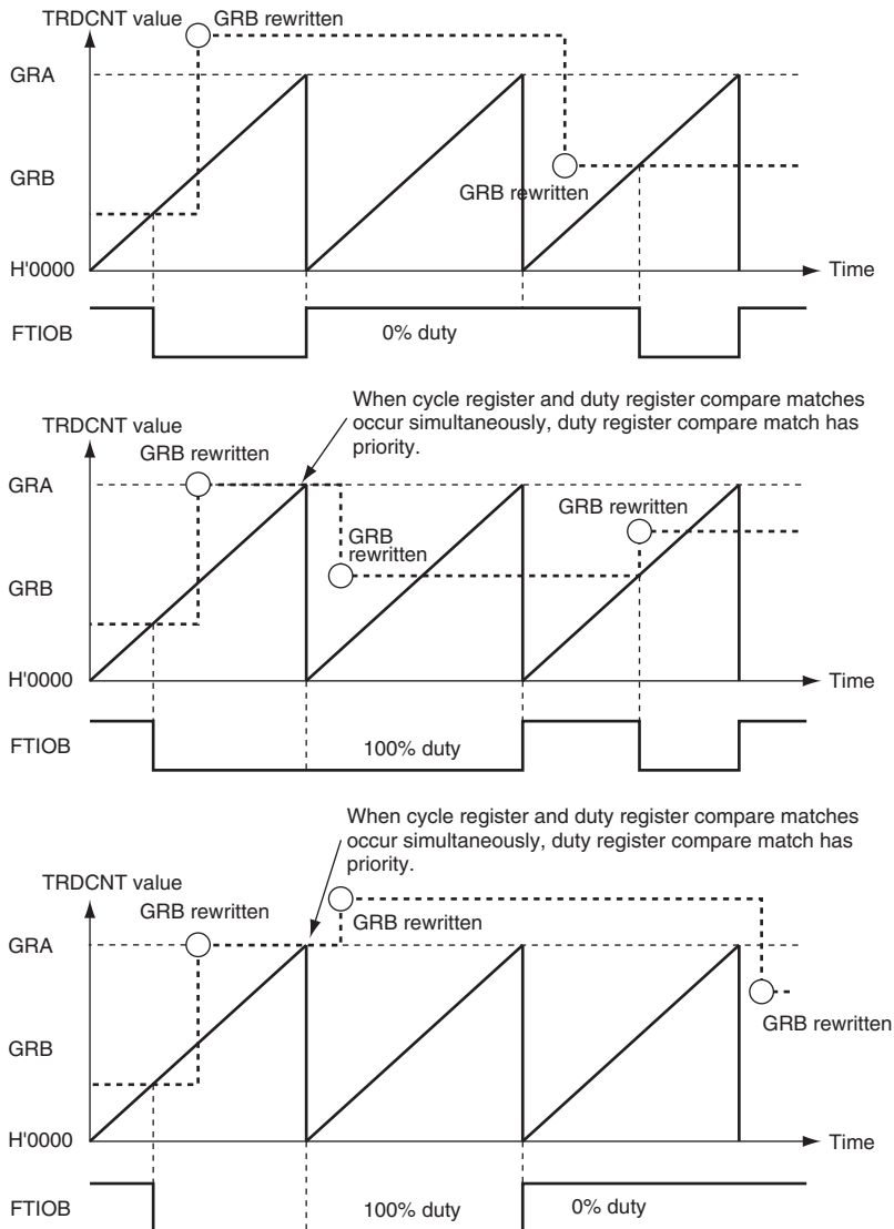
Figure 16.24 Example of PWM Mode Operation (3)
