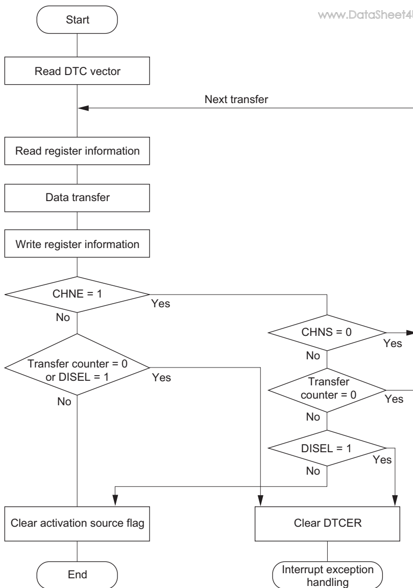
Figure 11.5 Flowchart of DTC Operation
