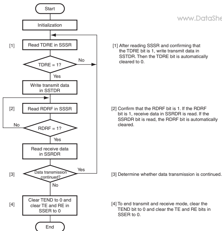
Figure 22.9 Sample Flowchart for Serial Transmit and Receive Operations
