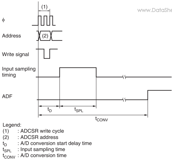
Figure 24.7 A/D Conversion Timing
