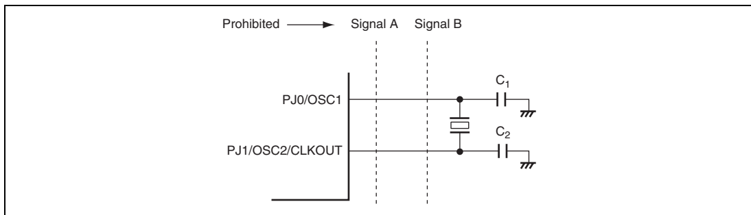
Figure 5.23 Example of Incorrect Board Design
