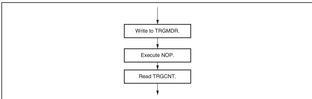
Figure 18.1 Timer RG Block Diagram
