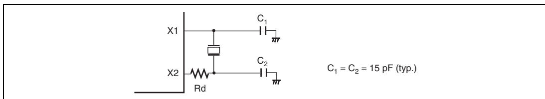
Figure 5.21 Typical Connection to 32.768-kHz Crystal Resonator
