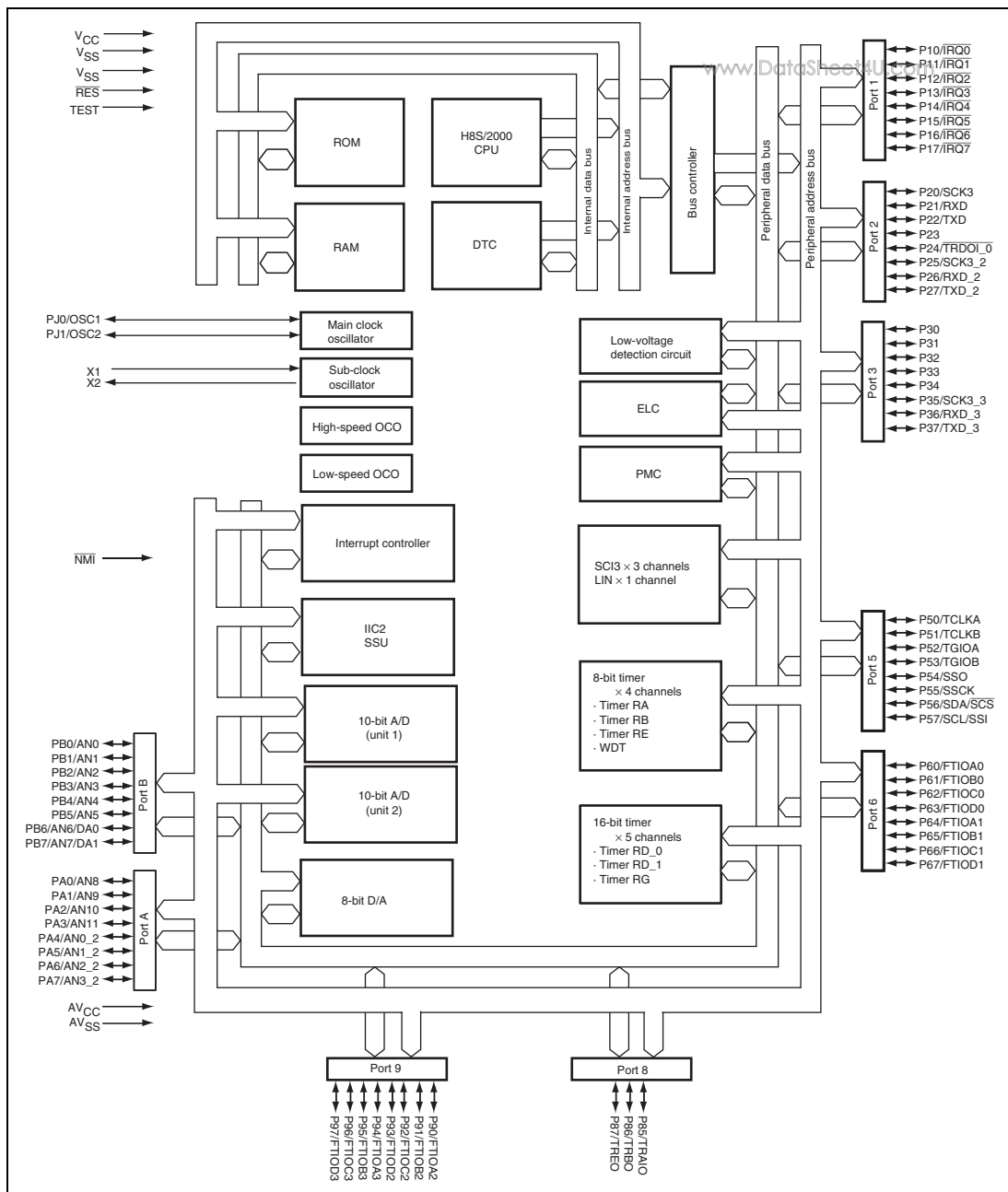
Figure 1.4 Block Diagram of H8S/2023 Group
