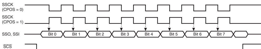
Figure 22.2 Relationship between Clock Polarity and Phase, and Data
