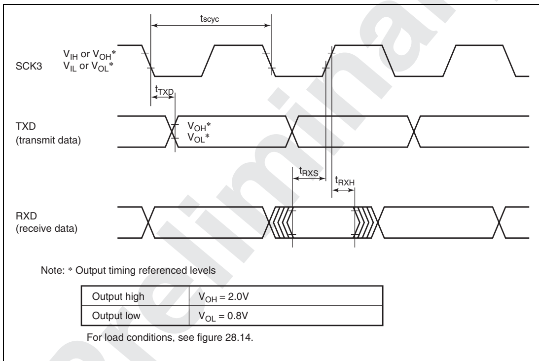
Figure 28.7 SCI Input/Output Timing in Clock Synchronous Mode
