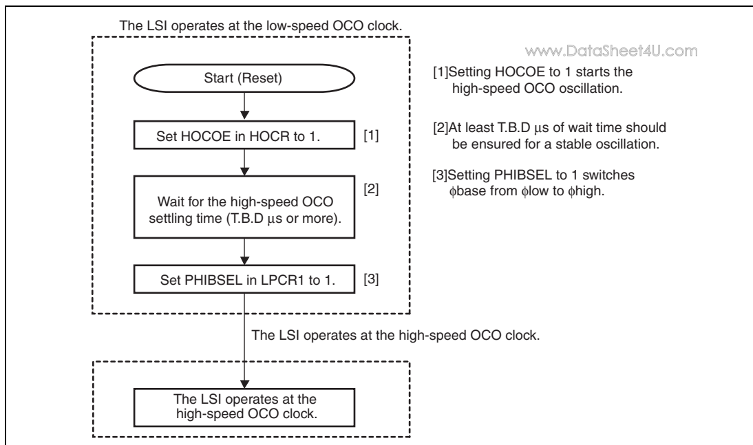
Figure 5.4 Flowchart for Ensuring Oscillation Settling Time by User and Switching from \phi_{\text{loco}} to High-Speed OCO
