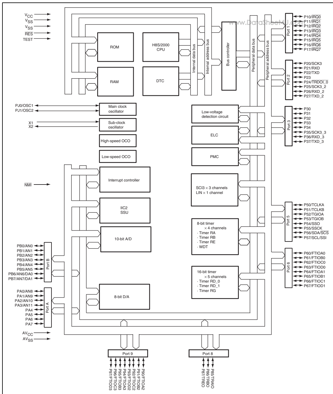
Figure 1.3 Block Diagram of H8S/20203 Group
