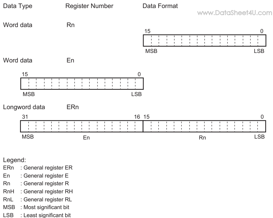
Figure 2.7 General Register Data Formats (2)
