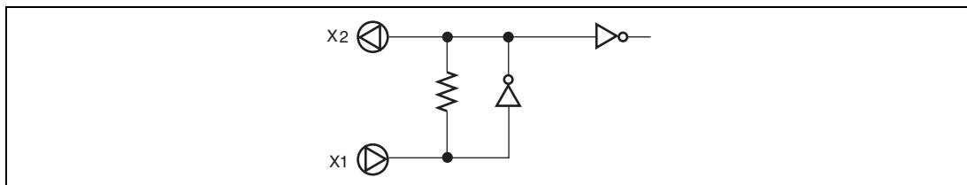
Figure 5.20 Block Diagram of Subclock Generator
