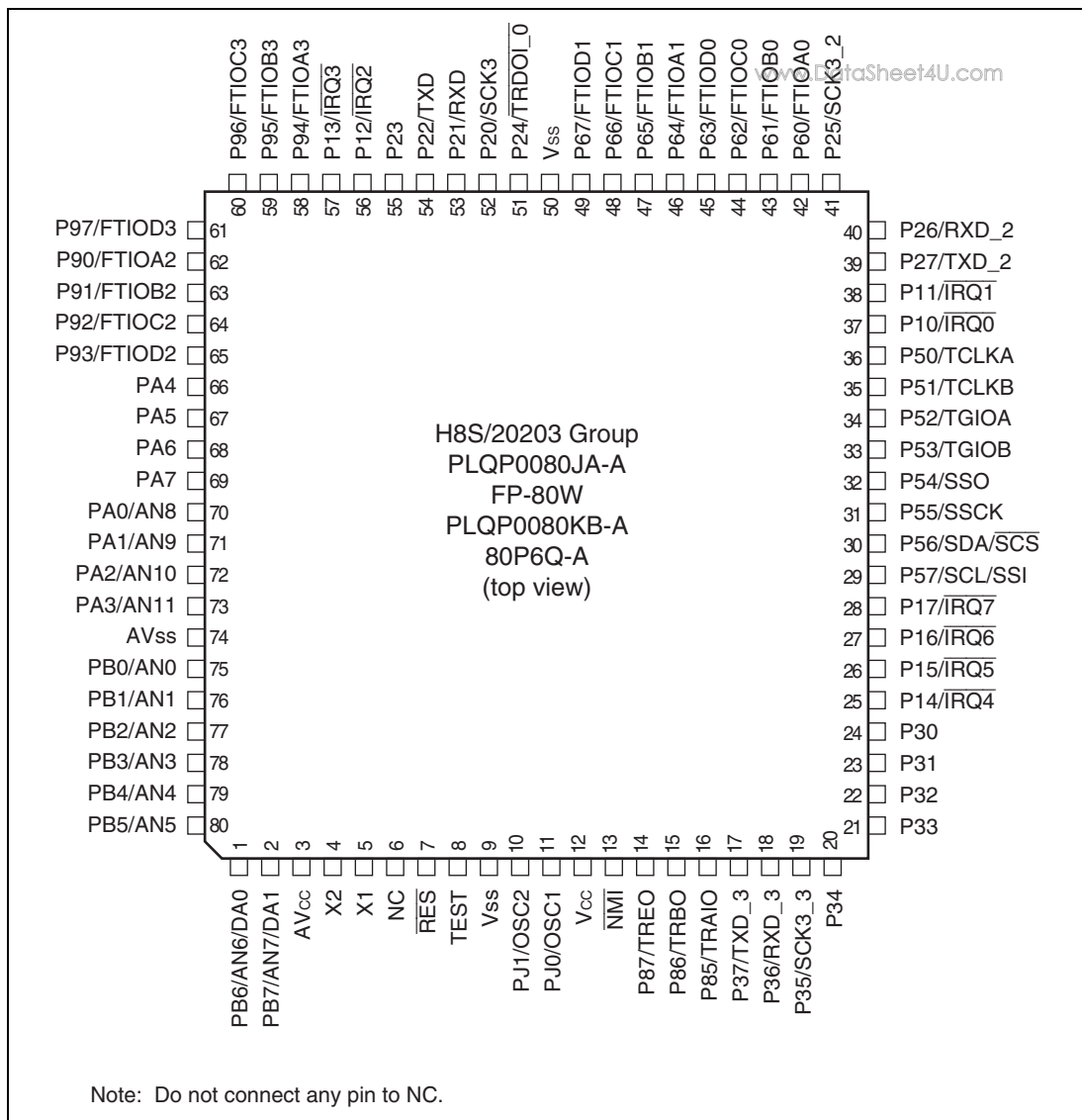
Figure 1.6 Pin Assignment of H8S/20203 Group
