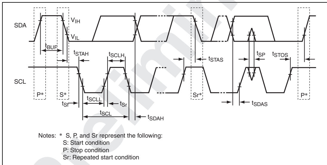
Figure 28.5 Timing of I 2 C Bus Interface Input/Output
