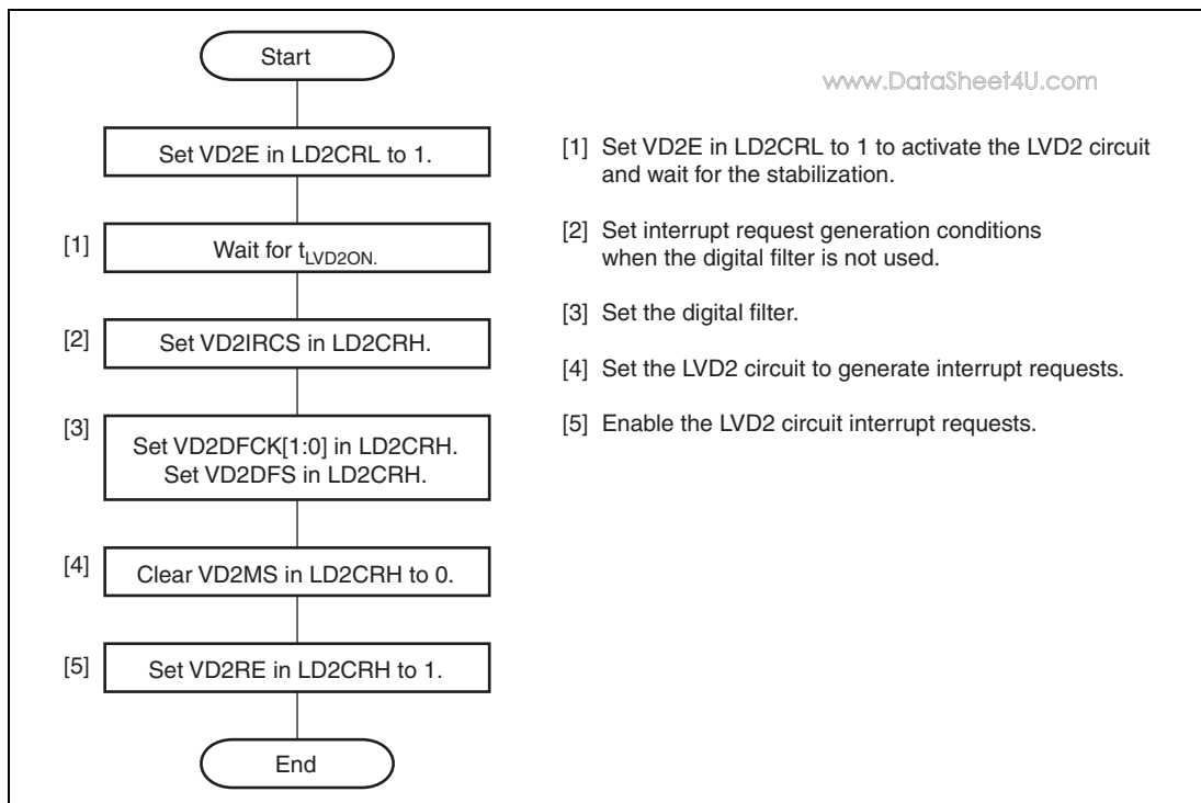
Figure 26.9 Procedure to Set LVDR2
