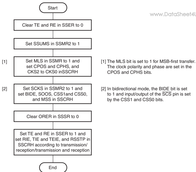
Figure 22.10 Initialization in Four-Line Bus Communication Mode
