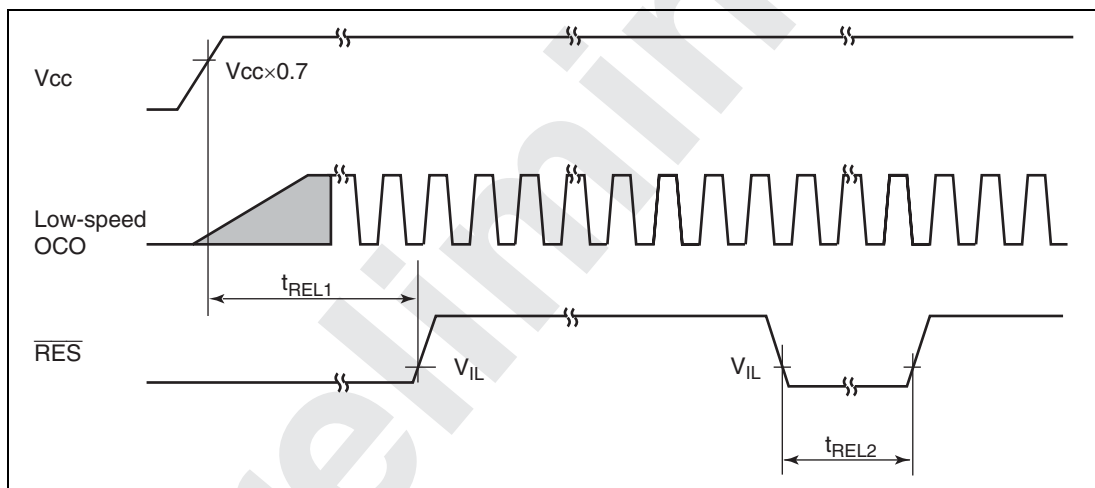
Figure 28.2 Timing of \overline{RES} Pin Low Width
