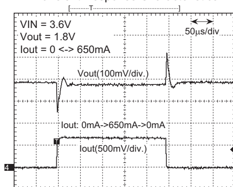
Transient Response Characteristics
