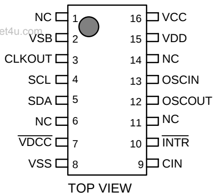
R2051Sxx(SSOP16)
