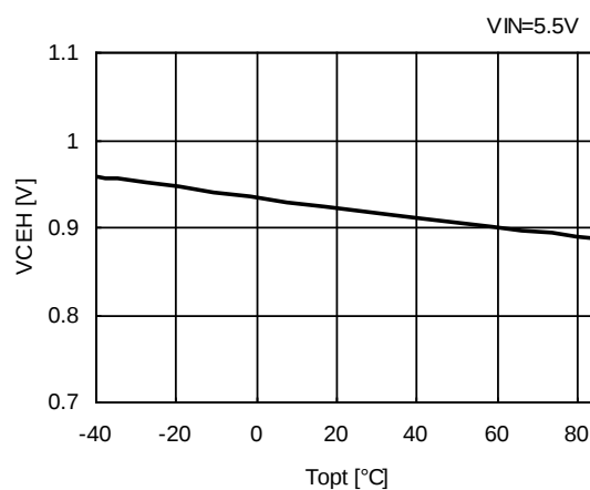
4) CE "H" Input Voltage vs. Temperature R1283x00xx
