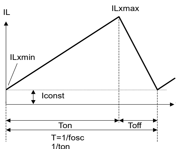
Continuous Mode
