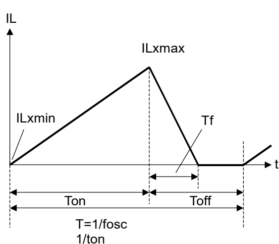
Discontinuous Mode
