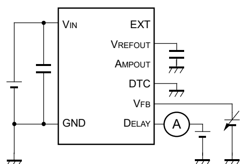
Fig. 4 D_{DELAY} Pin Charge Current/ Discharge Current Test Circuit
