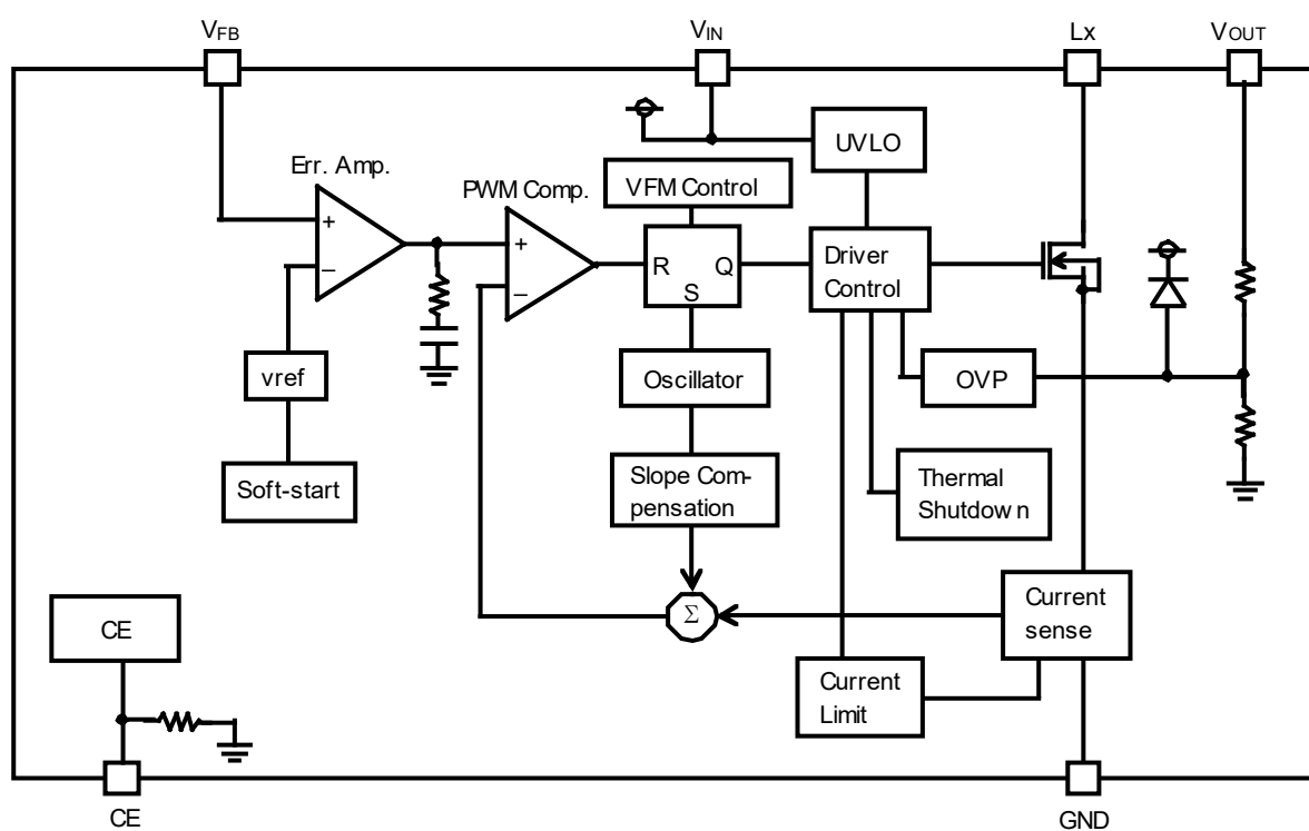
R1204xxxxC/F Block Diagram
