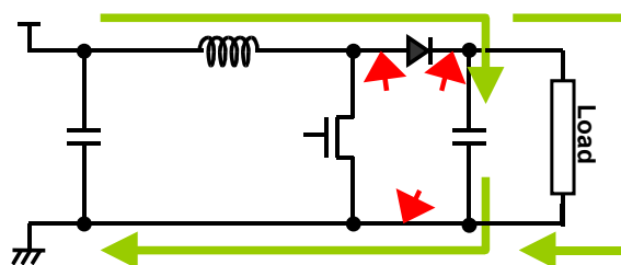
Figure 9. MOSFET-OFF
