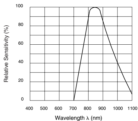
Fig. 5 Spectral Sensitivity
