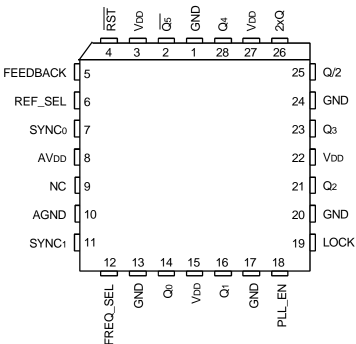
PLCC TOP VIEW
