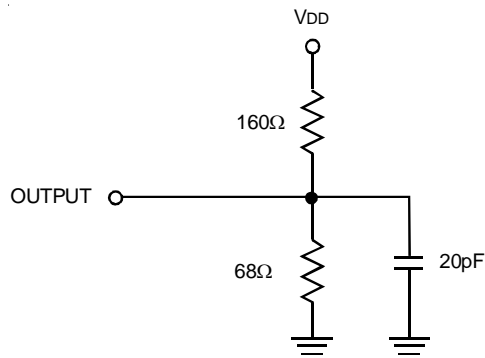
TEST CIRCUIT 1
