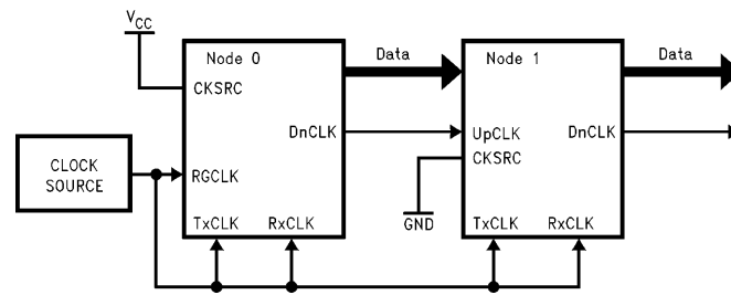
FIGURE 5.1. Recommended for Card-to-Card Connections Over QuickRing
