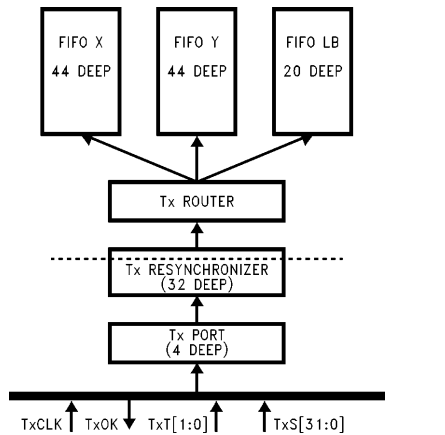
FIGURE 3.2. Tx Port Client Interface
