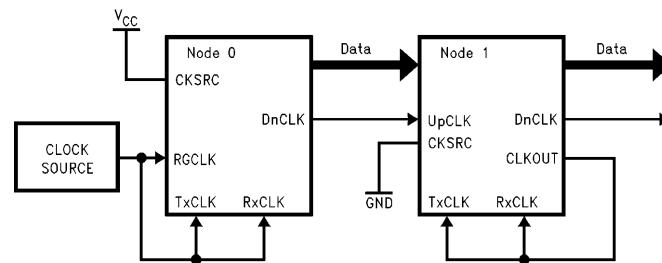
FIGURE 5.2. Recommended for Box-to-Box or Card-to-Card Connectors Over QuickRing
