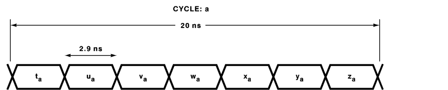
FIGURE 4.2. Seven Sub-Symbols in one Clock Cycle
