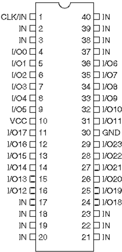
CERDIP
