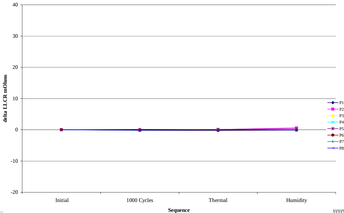
Board #4 Power Contacts
