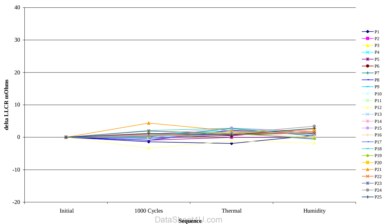
Board #5 Signal Contacts
