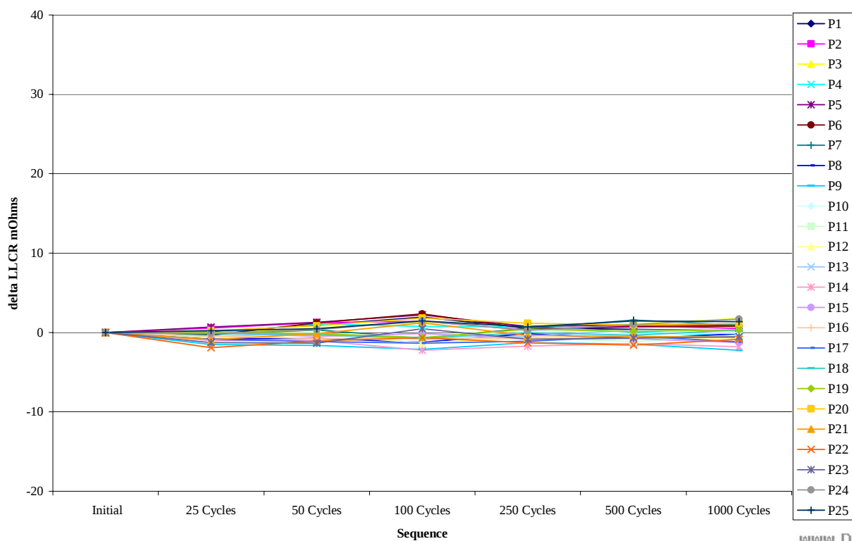
Board #7 Signal Contacts
