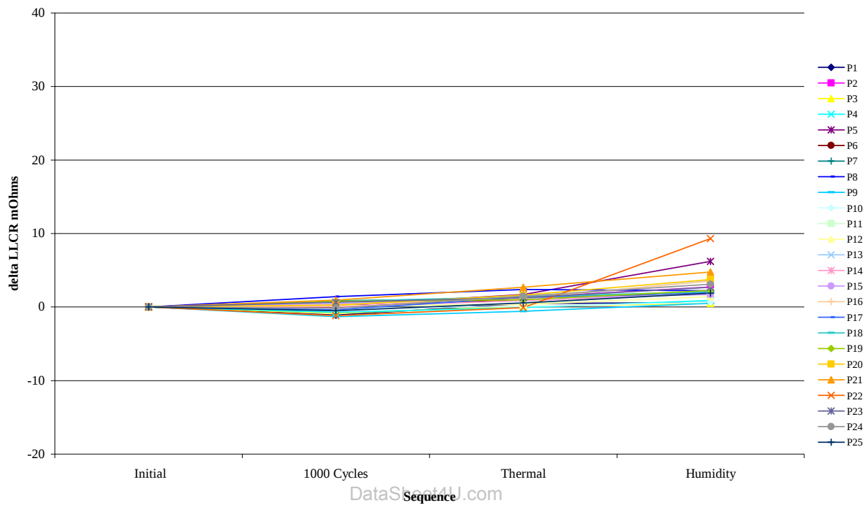
Board #3 Signal Contacts
