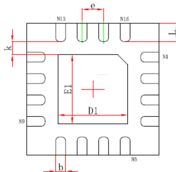
&lt;QFN -16&gt; Bottom View
