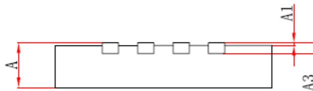
&lt;QFN -16&gt; Side View
